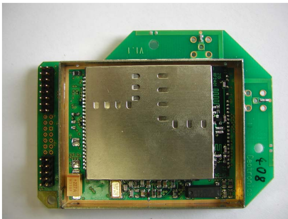
Photo 2: CT-DECT-H24 Headset / Top View Without Screening Plate
