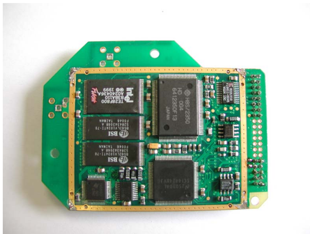
Photo 5: CT-DECT-I24 / Rear View Without Screening Plate
