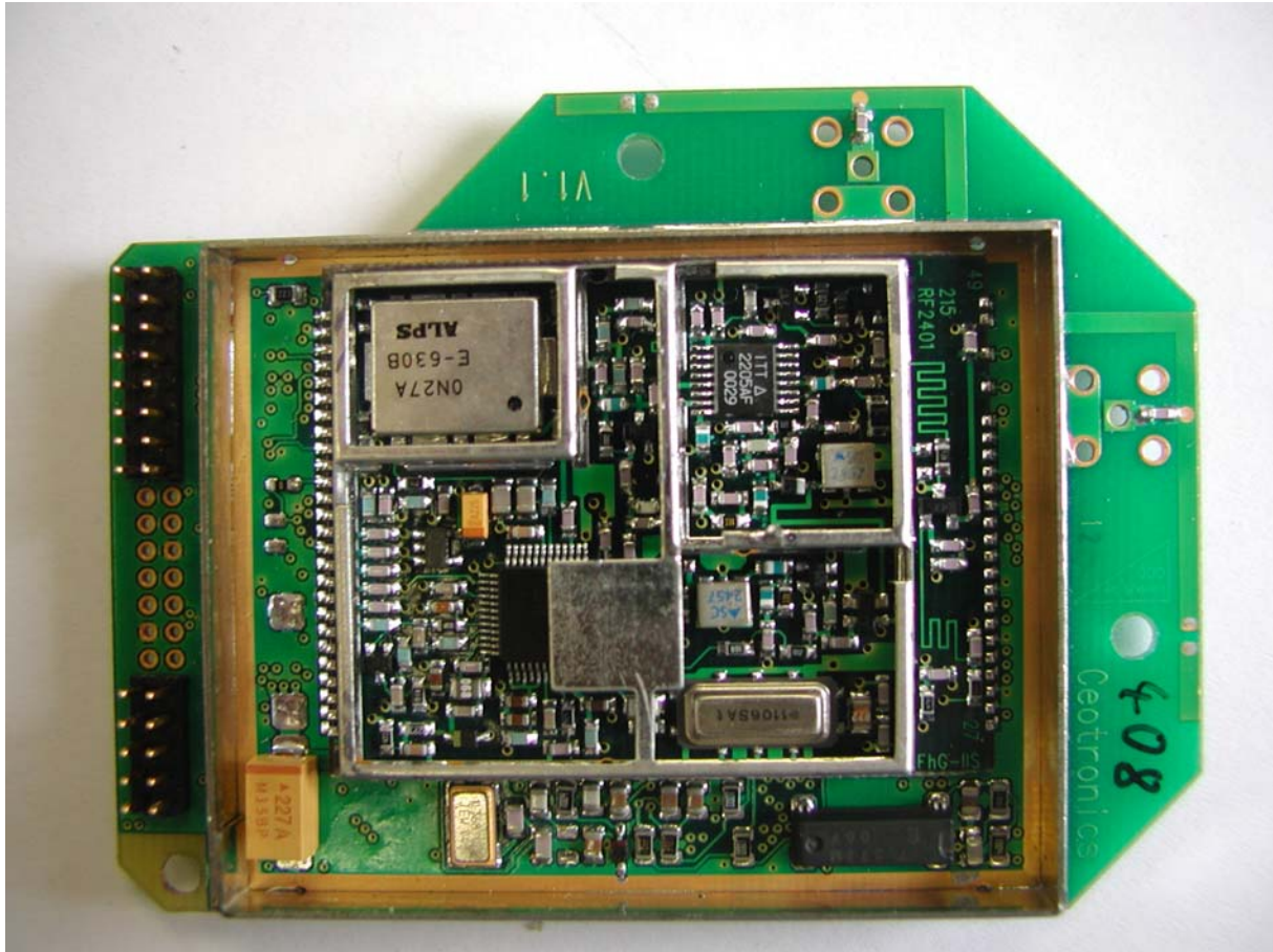
Photo 3: CT-DECT-I24 / Top View Without RF Screening Plate
