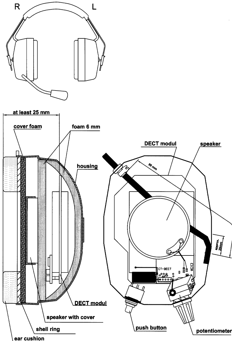
Fig. 1: Module Position Inside The Headset
