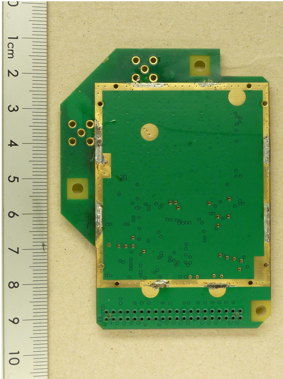
134429_16.JPG: DECT module, shielding removed, bottom view
