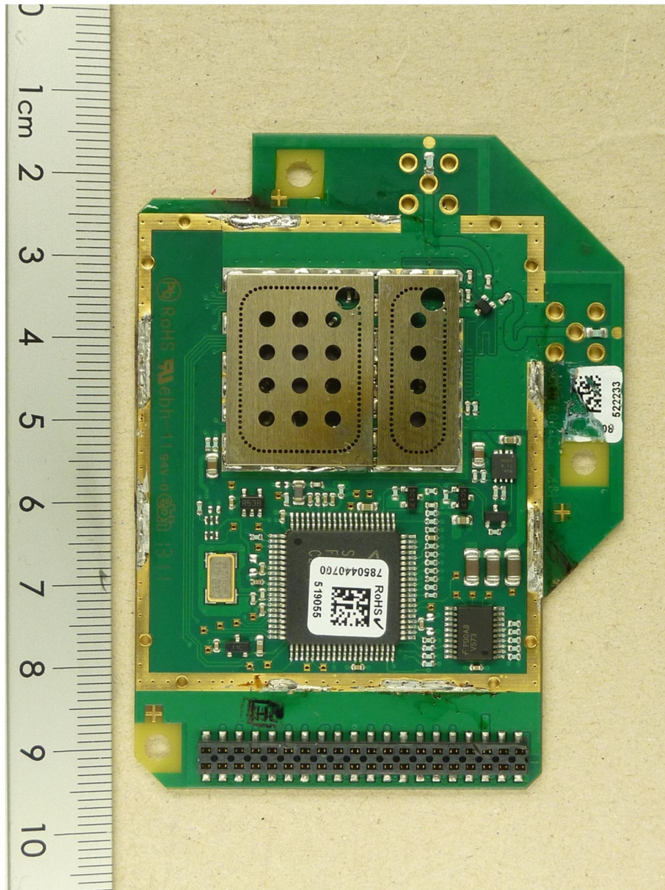
134429_14.JPG: DECT module, outer shielding removed, top view
