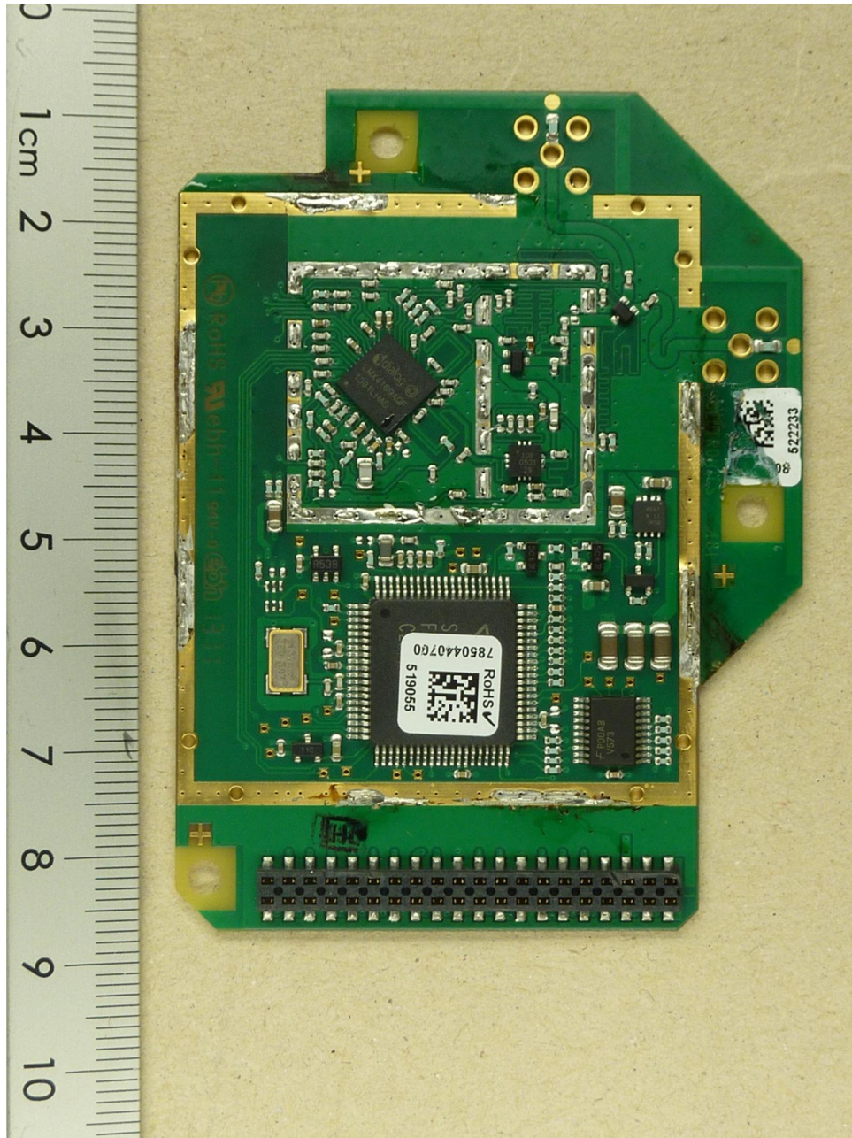
134429_15.JPG: DECT module, inner shielding removed, top view
