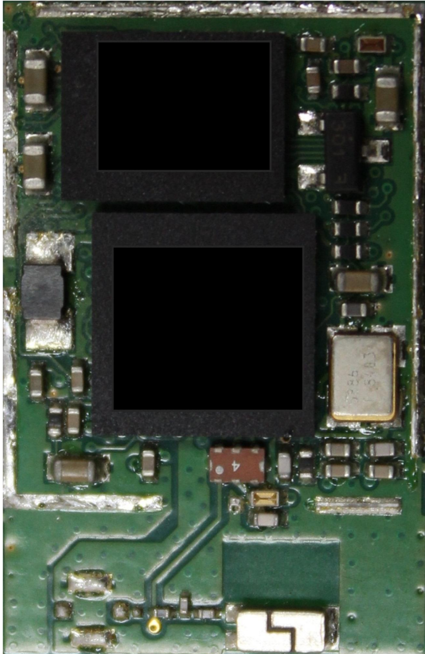
134429_17.JPG: Bluetooth module, shielding removed, top view
