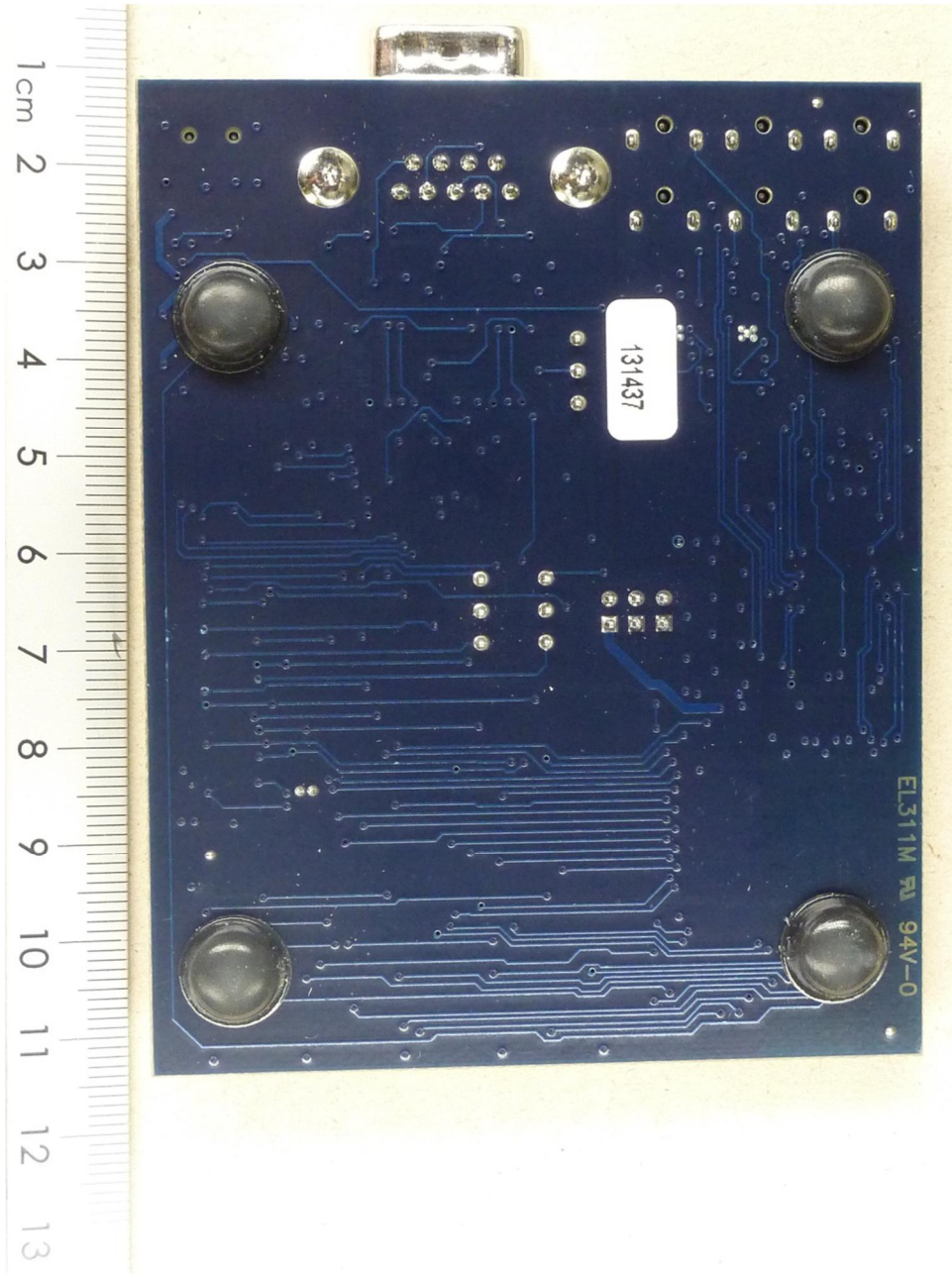
134429_13.JPG: Bluetooth evaluation board, bottom view
