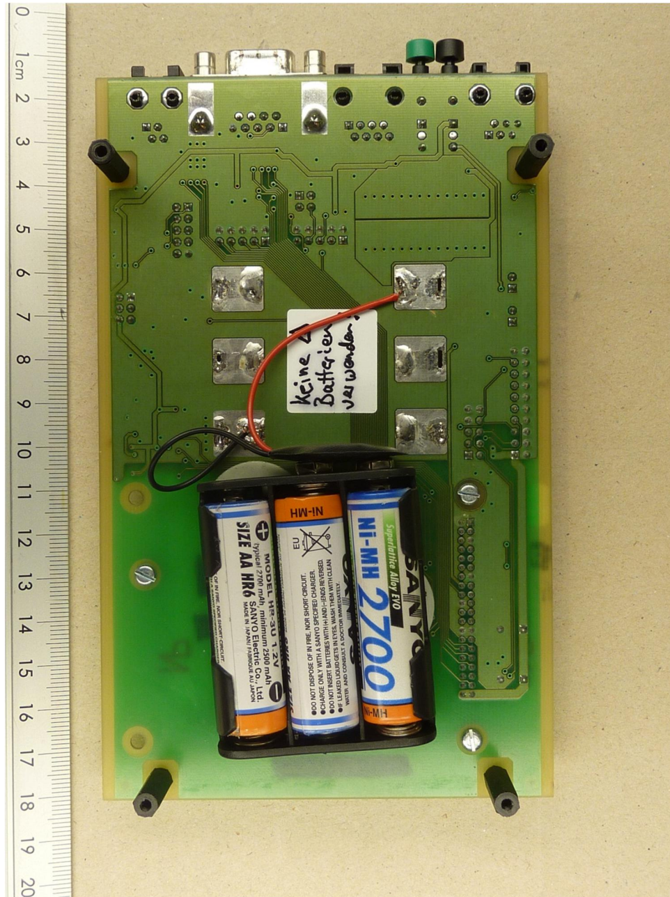
134429_10.JPG: DECT evaluation board, bottom view
