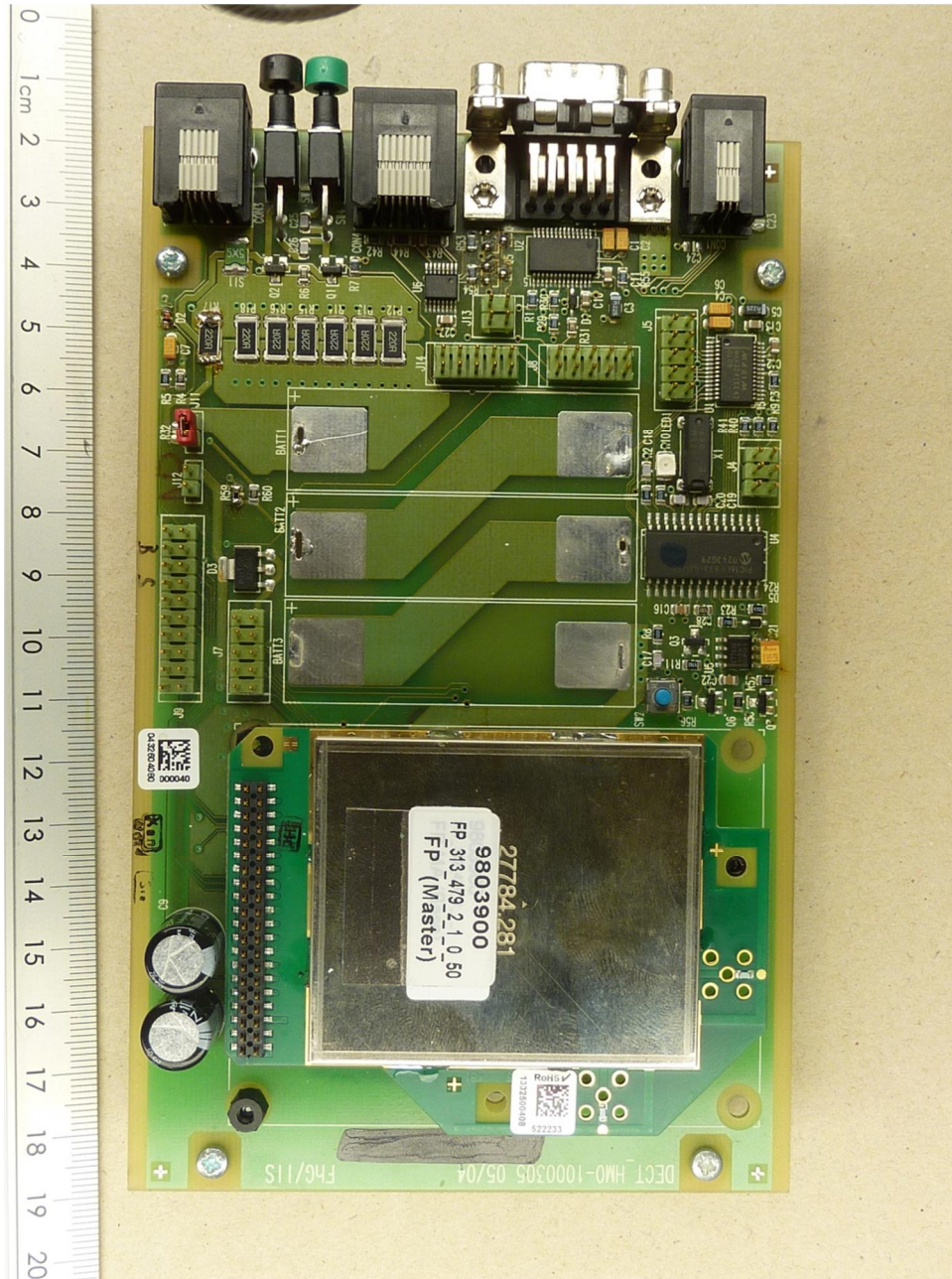
134429_9.JPG: DECT evaluation board, top view
