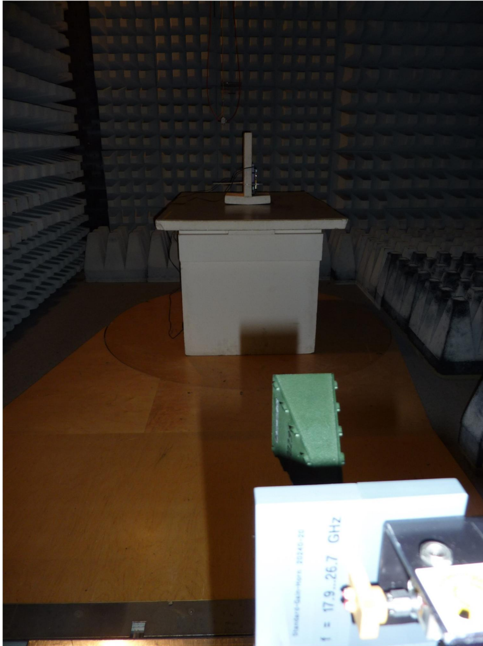
134429_4.JPG: Test setup fully anechoic chamber
