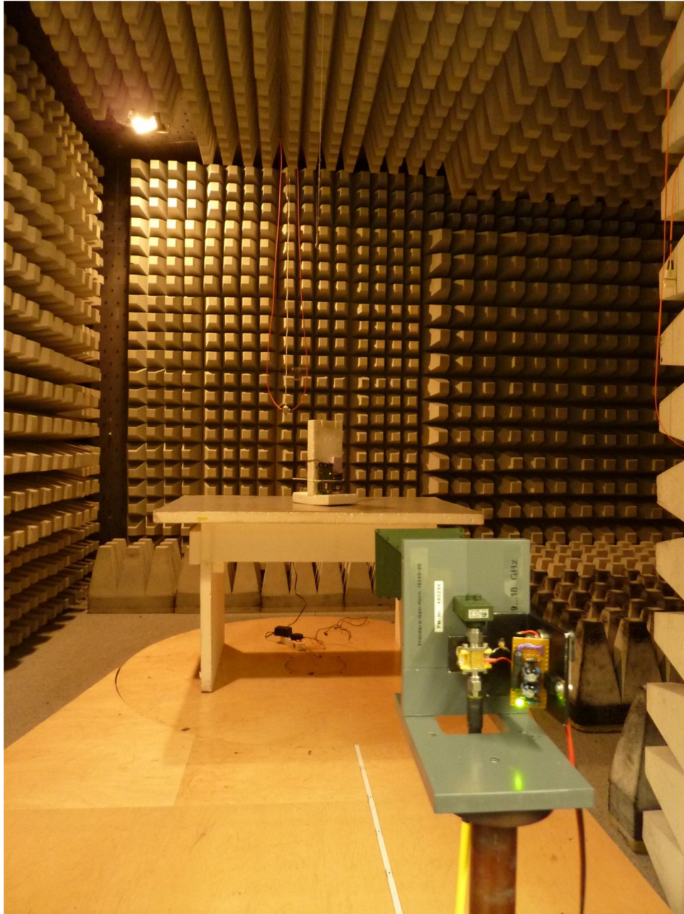
134429_3.JPG: Test setup fully anechoic chamber
