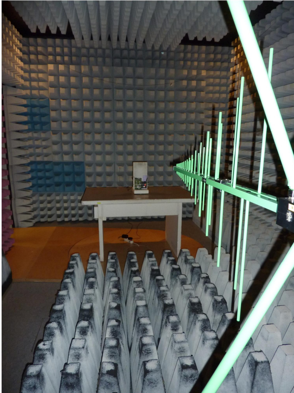
134429_1.JPG: Test setup fully anechoic chamber
