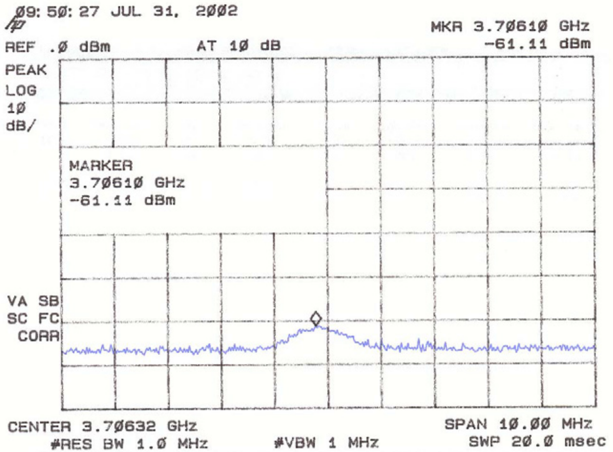
Figure 5k Peak Radiated Spurious Emission 15.247(c) - High
