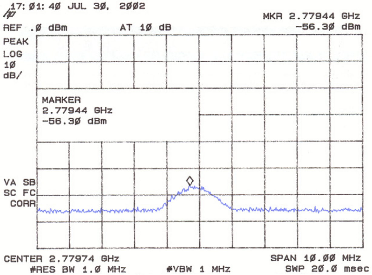
Figure 5j Peak Radiated Spurious Emission 15.247(c) - High
