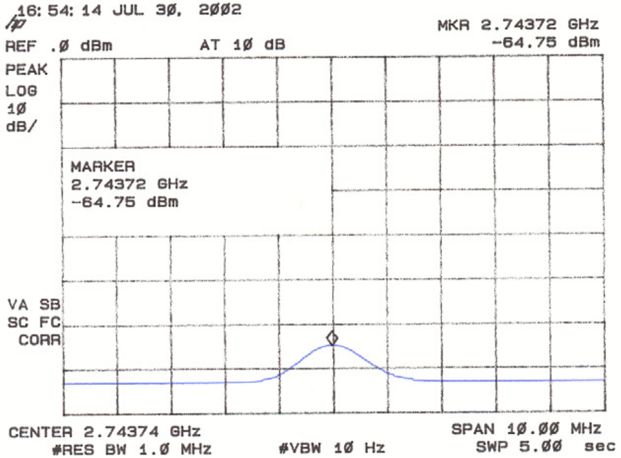
Figure 6b Average Radiated Spurious Emission 15.247(c) - Mid
