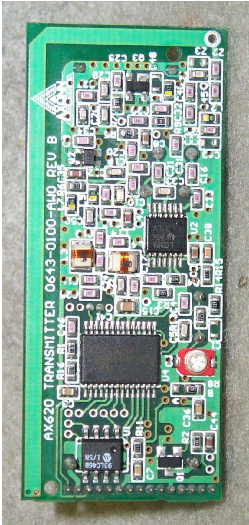
Photo 4. EUT, Top View
