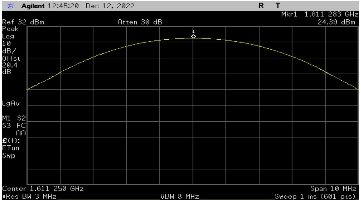
Plot 1 – Output Power – Low Channel
