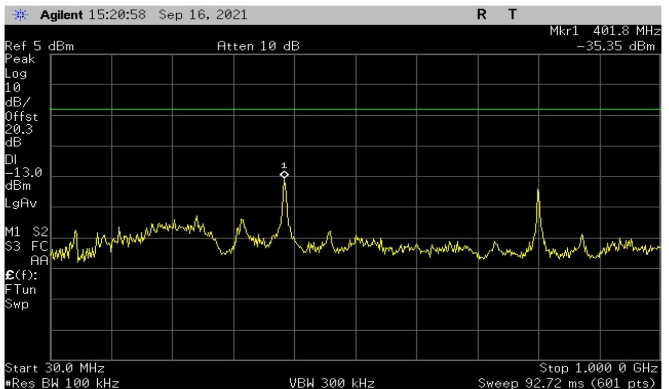
Plot 8 – Lowest Channel - 30MHz to 1GHz
