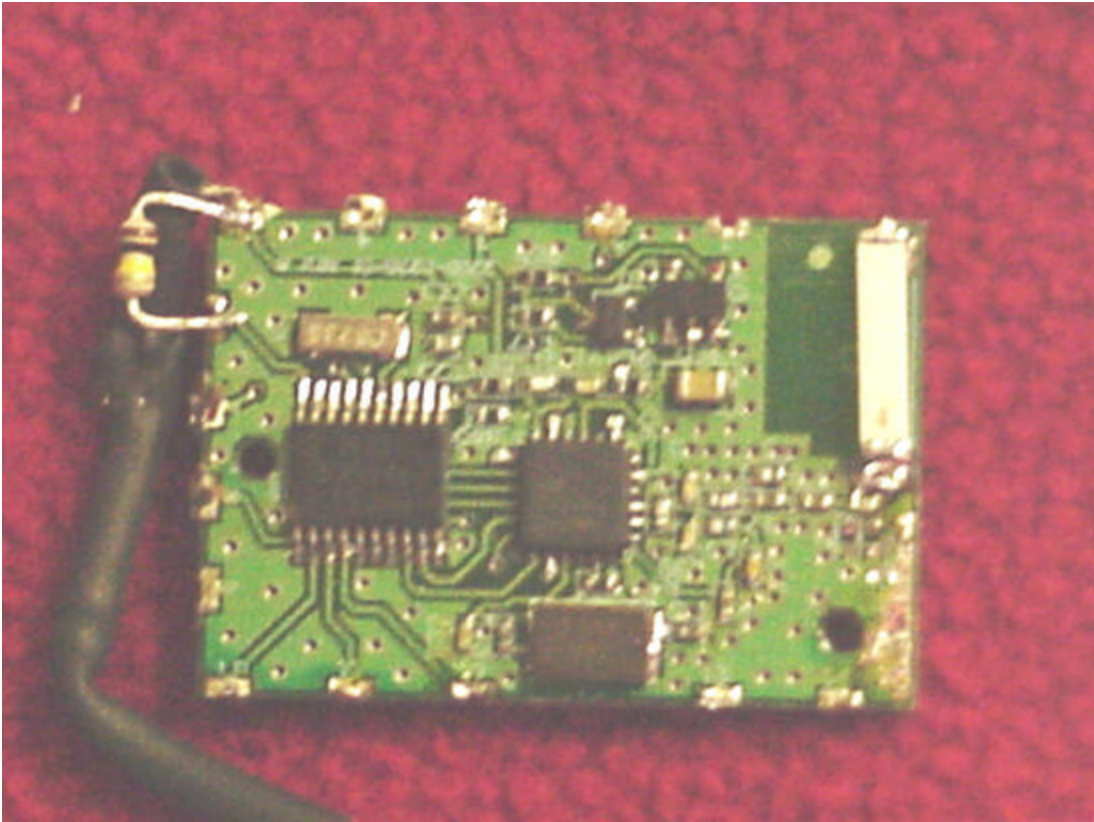
Photo 5. Component Side EUT
