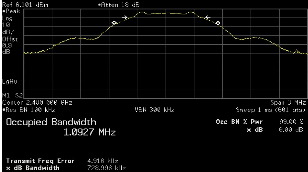
Plot 5 – Highest Channel – 6dB BW
