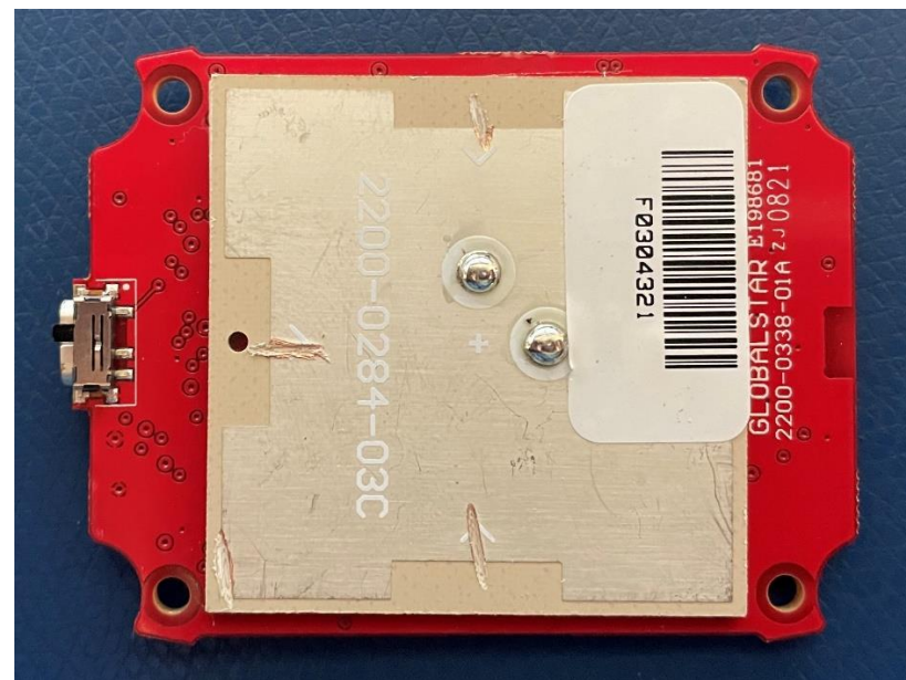
S1C PCB – Antenna Side
