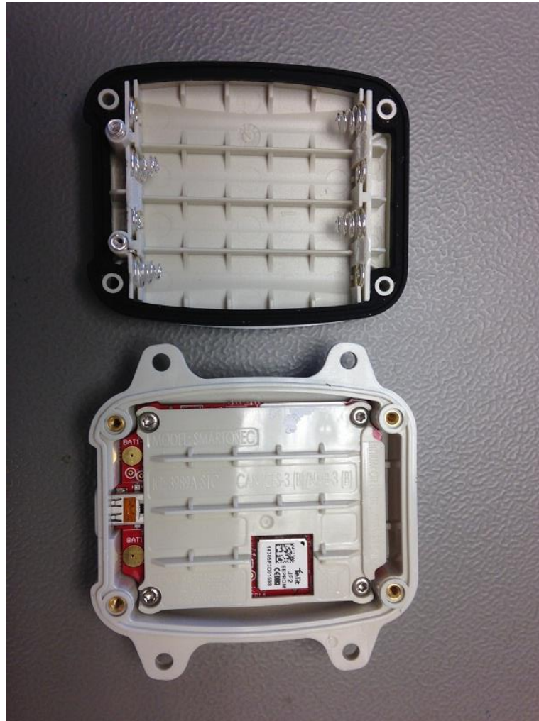
S1C Opened with batteries removed
