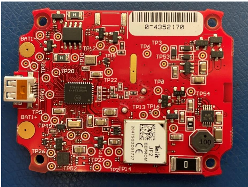
S1C PCB – Component Side
