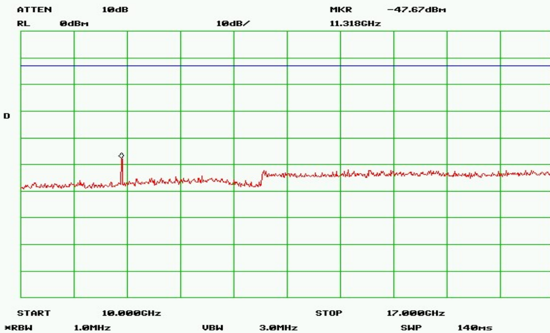
Plot 16 Highest Channel - 10GHz to 17GHz
