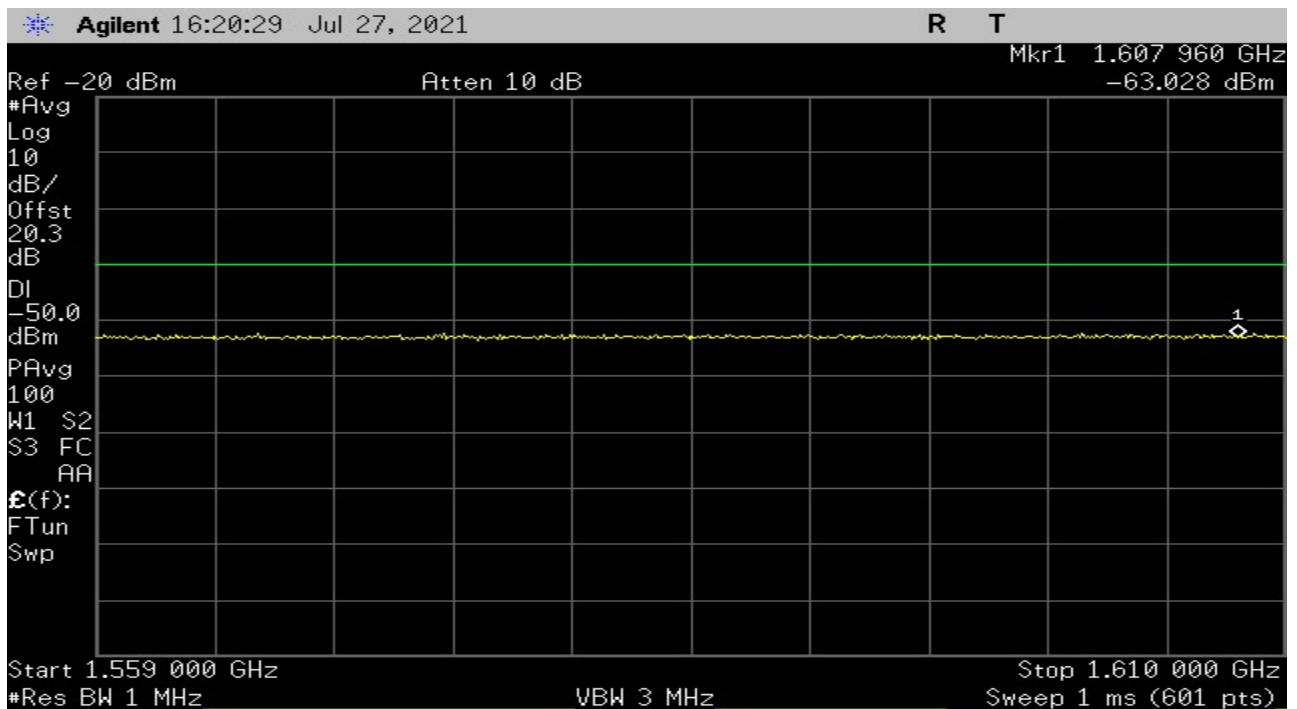
Plot 26 – High Channel – Carrier Off
