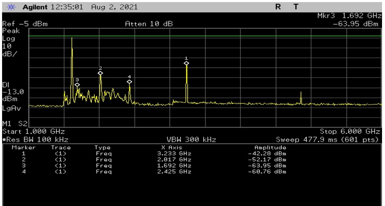
Plot 14 Highest Channel - 1GHz to 6GHz
