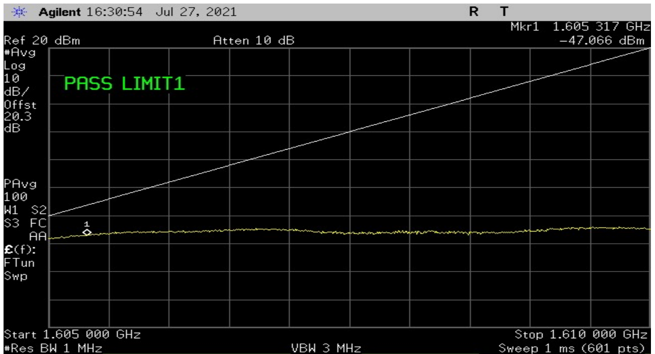
Plot 24-High Channel – Test Limit 25.216 (f)(g)
