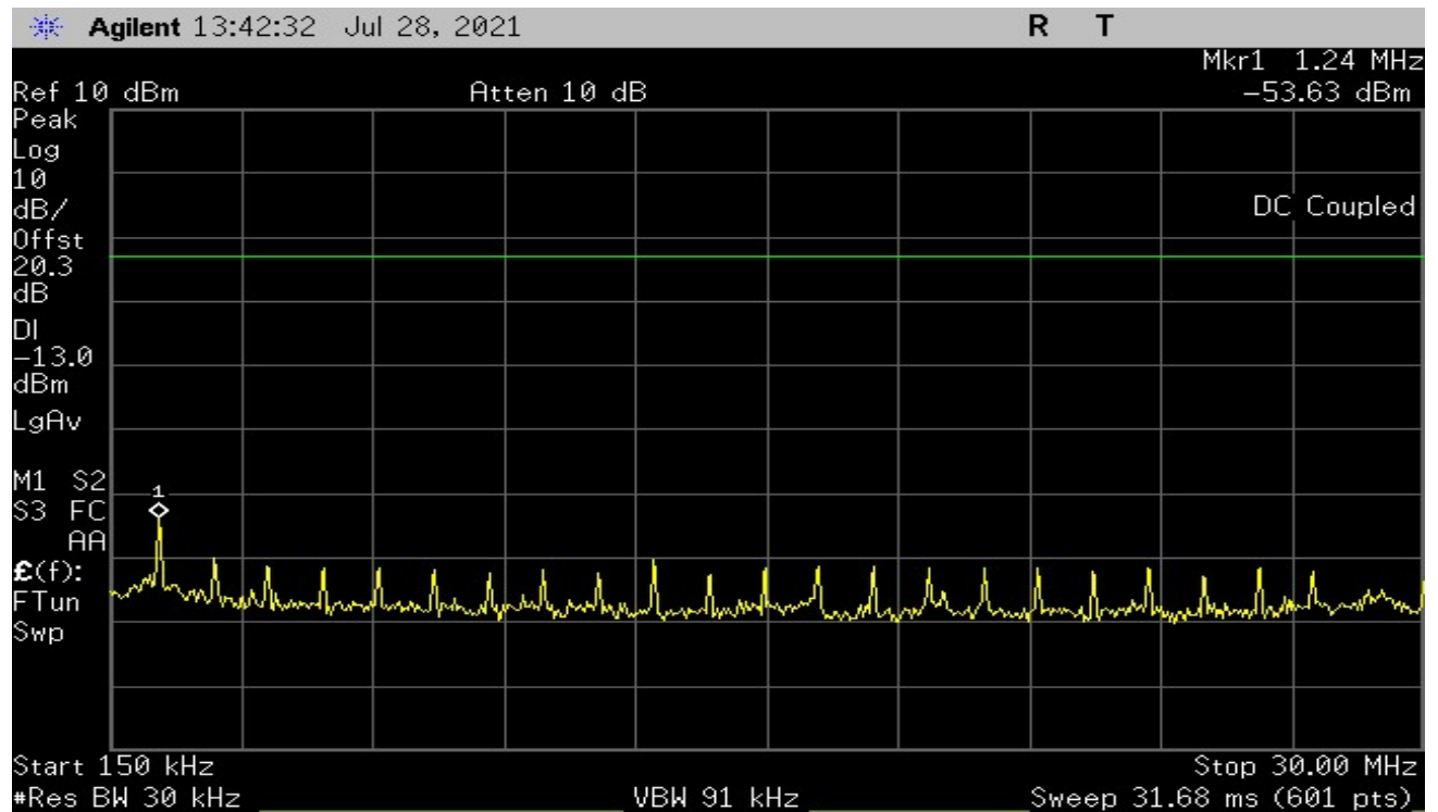
Plot 12 – Highest Channel – 150kHz to 30MHz
