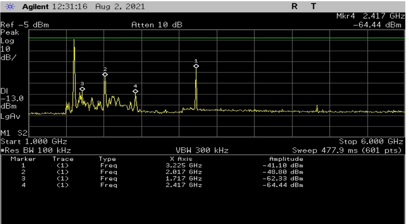
Plot 9 – Lowest Channel - 1GHz to 6GHz
