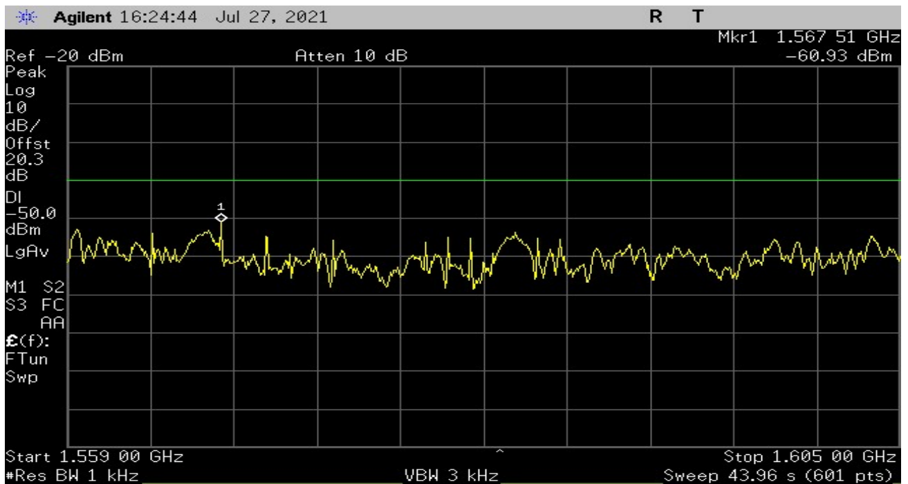
Plot 18 – High Channel – Test Limit 25.216 (c) – Discrete Emissions
