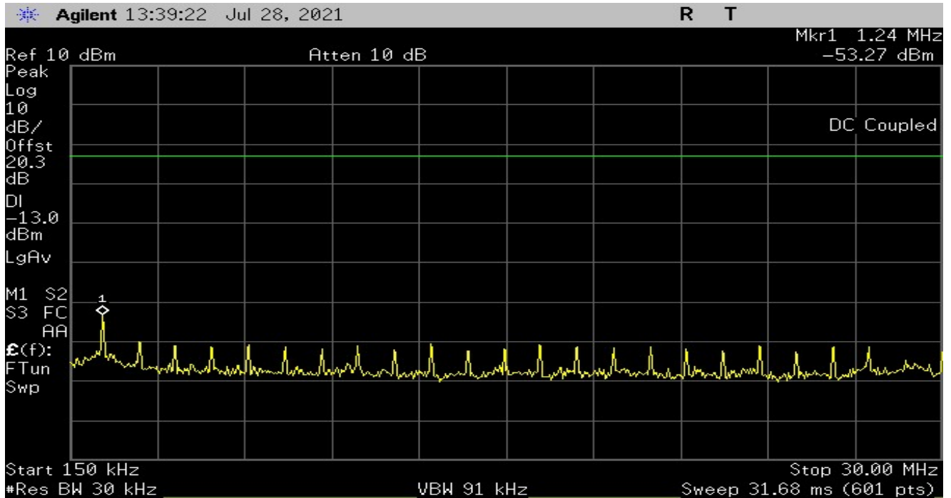
Plot 7 – Lowest Channel - 150kHz to 30MHz
