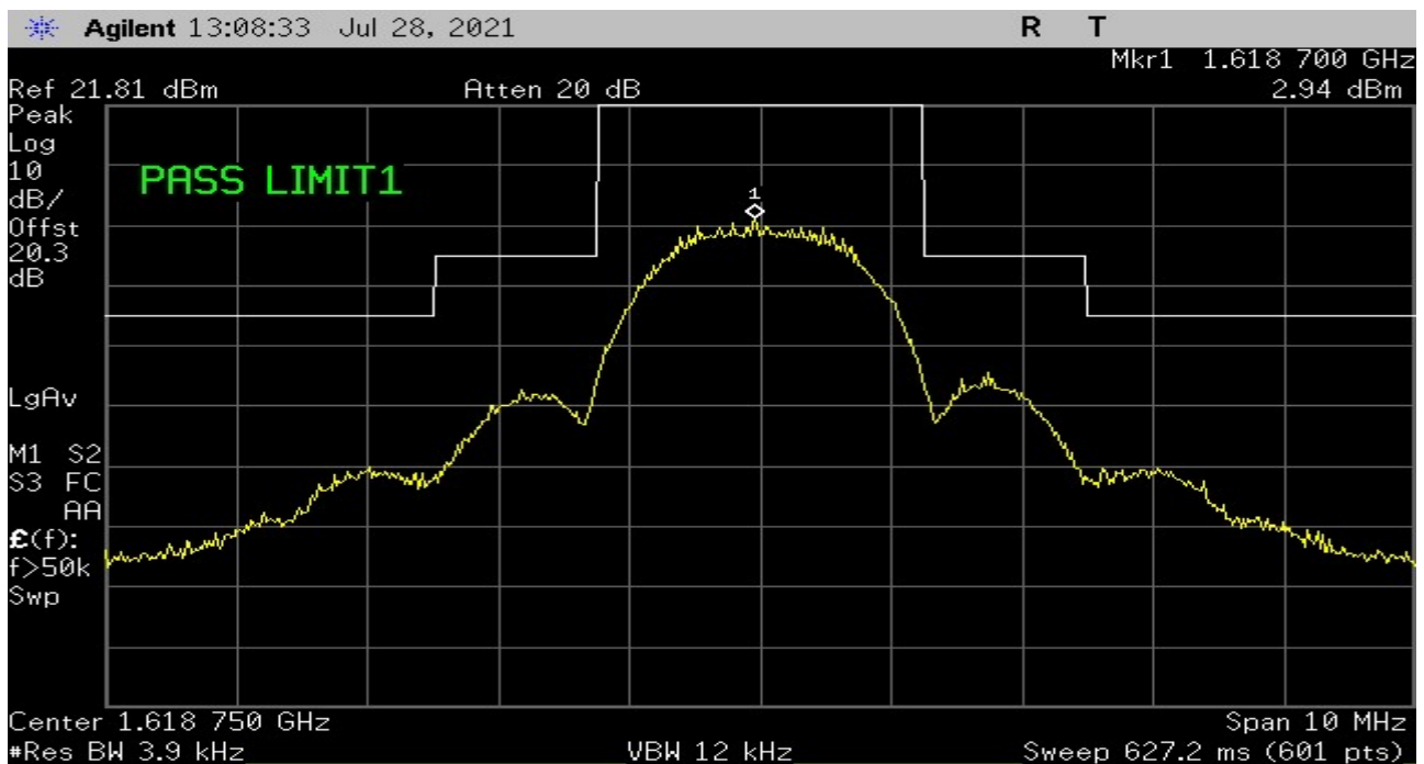
Plot 6 – Emission Mask - High Channel
