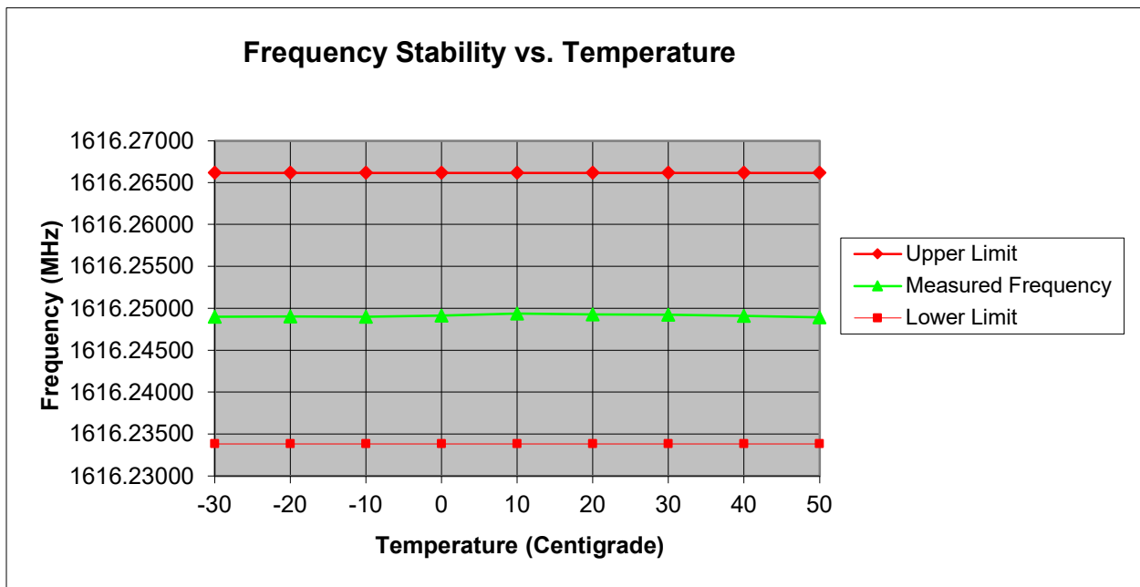
Plot 27 – Temperature vs Frequency
