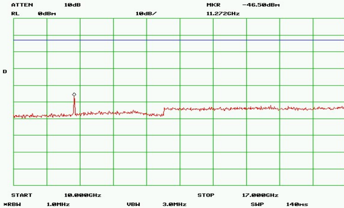
Plot 11 – Lowest Channel - 10GHz to 17GHz
