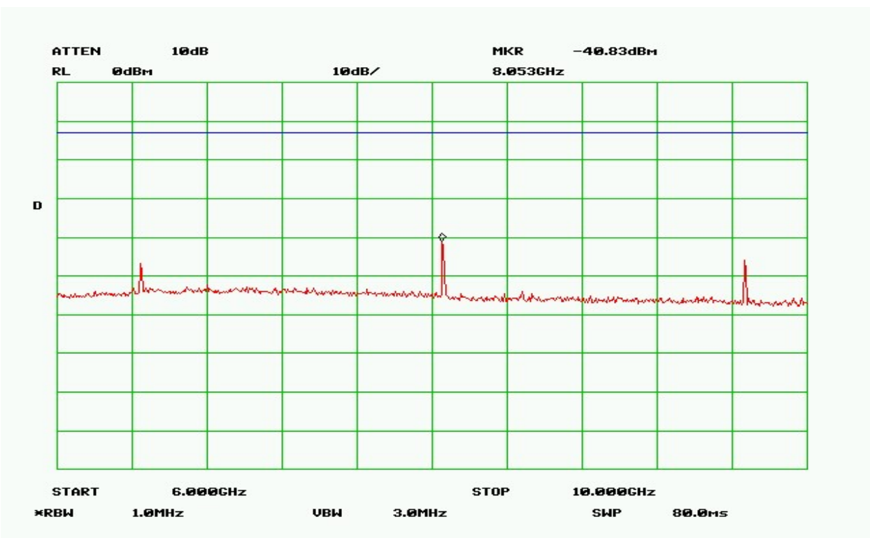
Plot 10 – Lowest Channel - 6GHz to 10 GHz
