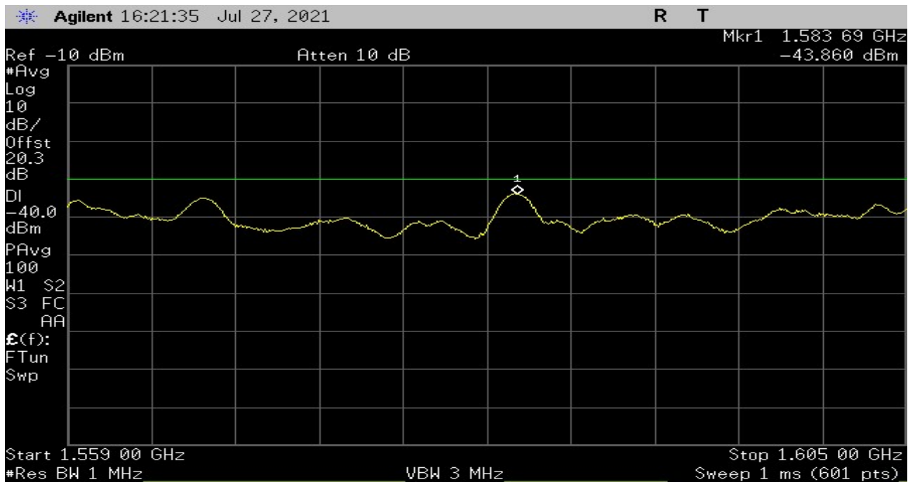
Plot 20 – High Channel – Test Limit 25.216 (c)
