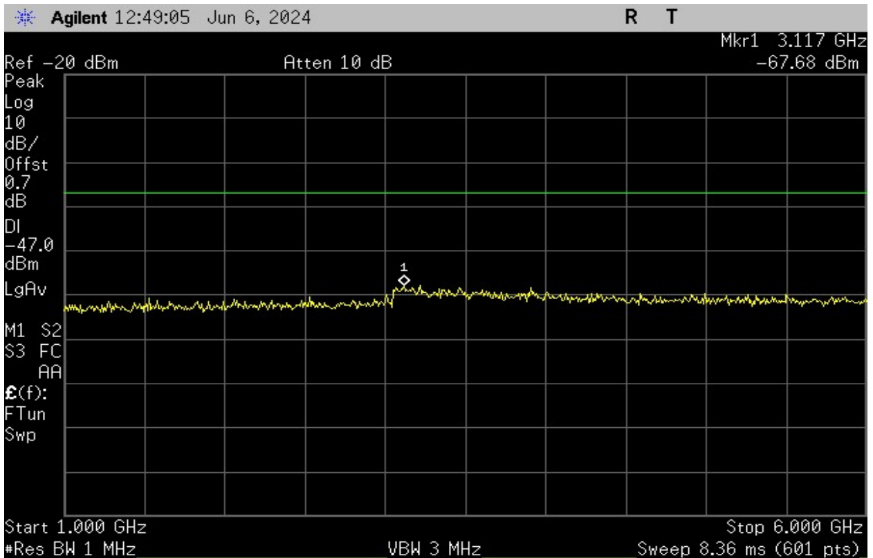
Plot 2 – Receiver Emissions (Conducted) – 1GHz to 6GHz (For Industry Canada RSS-GEN)
