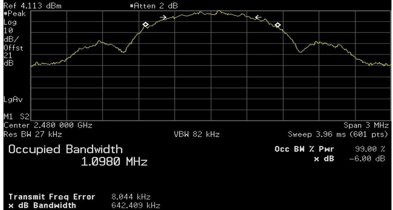
Plot 5 – Highest Channel – 6dB BW
