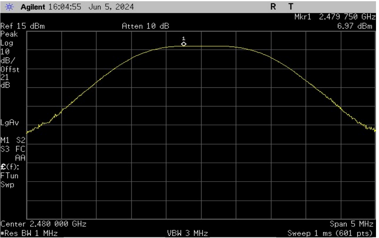
Plot 8 – Output Power – Highest Channel
