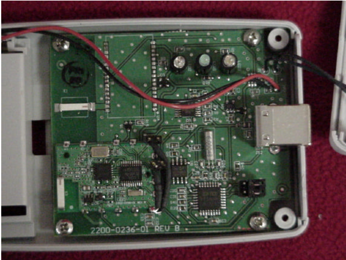
Photo 3. Close up View of Transmitter mounted on EUT Board
