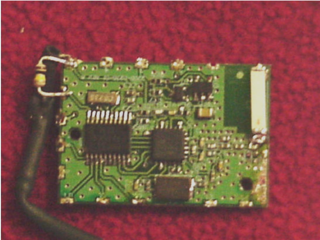
Photo 5. Component Side Transmitter
