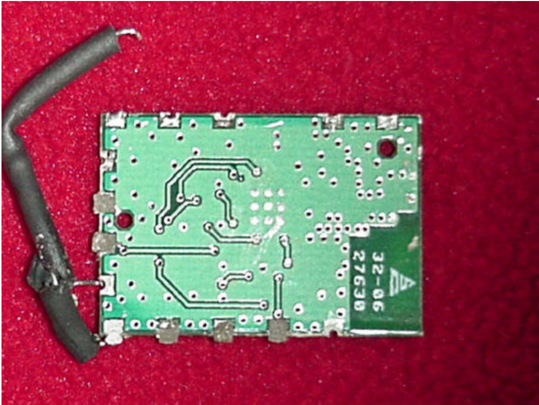
Photo 4. Solder Side of Transmitter
