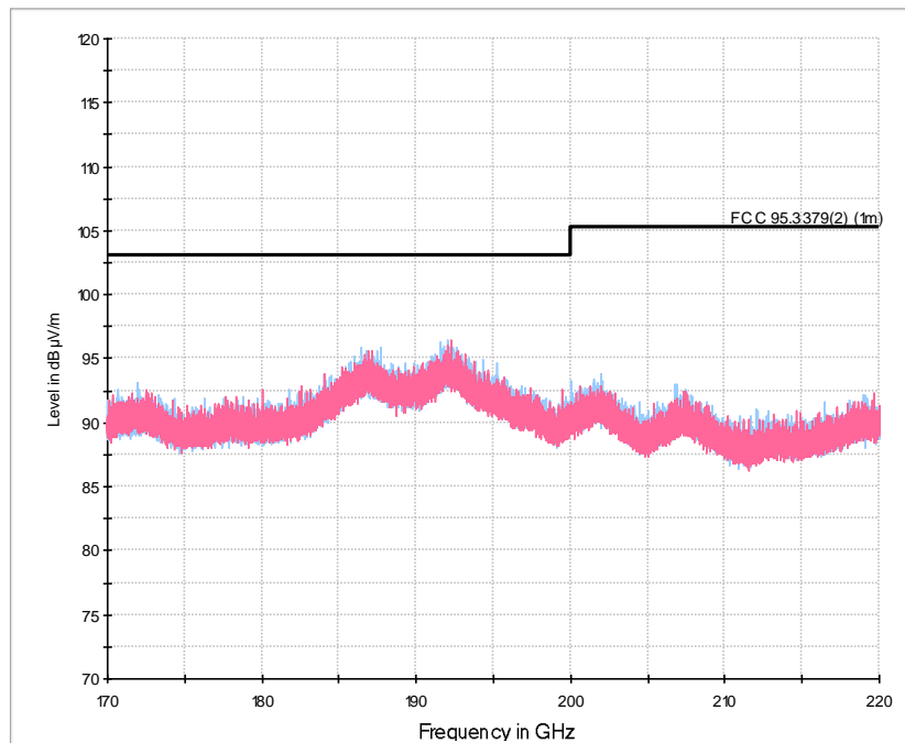
— Preview Result 1H-PK+ — Preview Result 1V-PK+ — FCC 95.3379(2) (µm) ◆ Final_Result PK+
