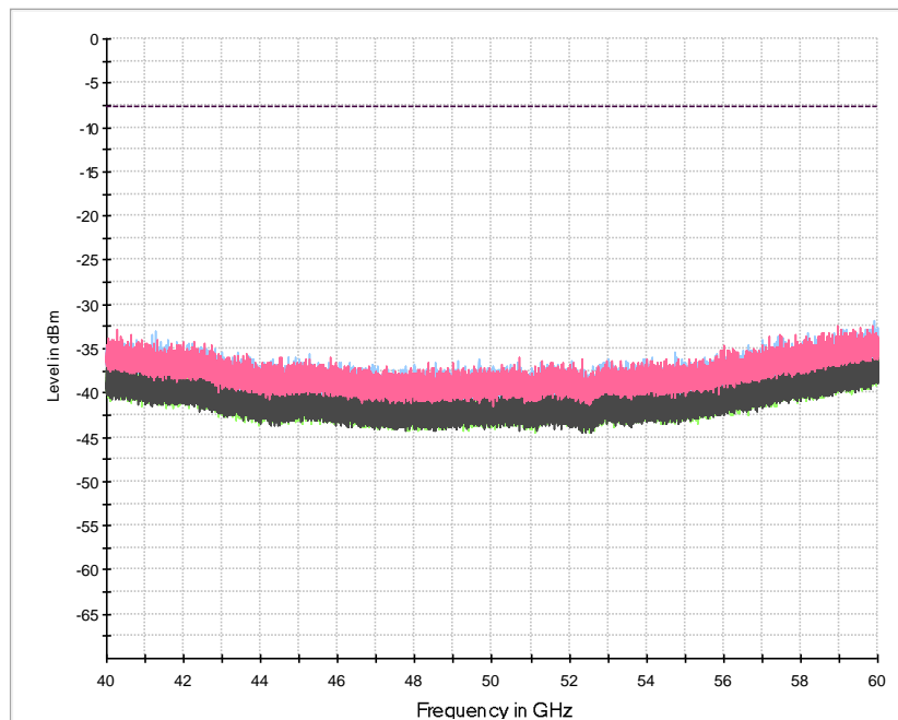
— Preview Result 2H-RMS — Preview Result 1H-PK+ — Preview Result 2V-RMS — Preview Result 1V-PK+ - - - FCC 95.3379(2) dBm ◆ Final_Result PK+ ◆ Final_Result RMS
