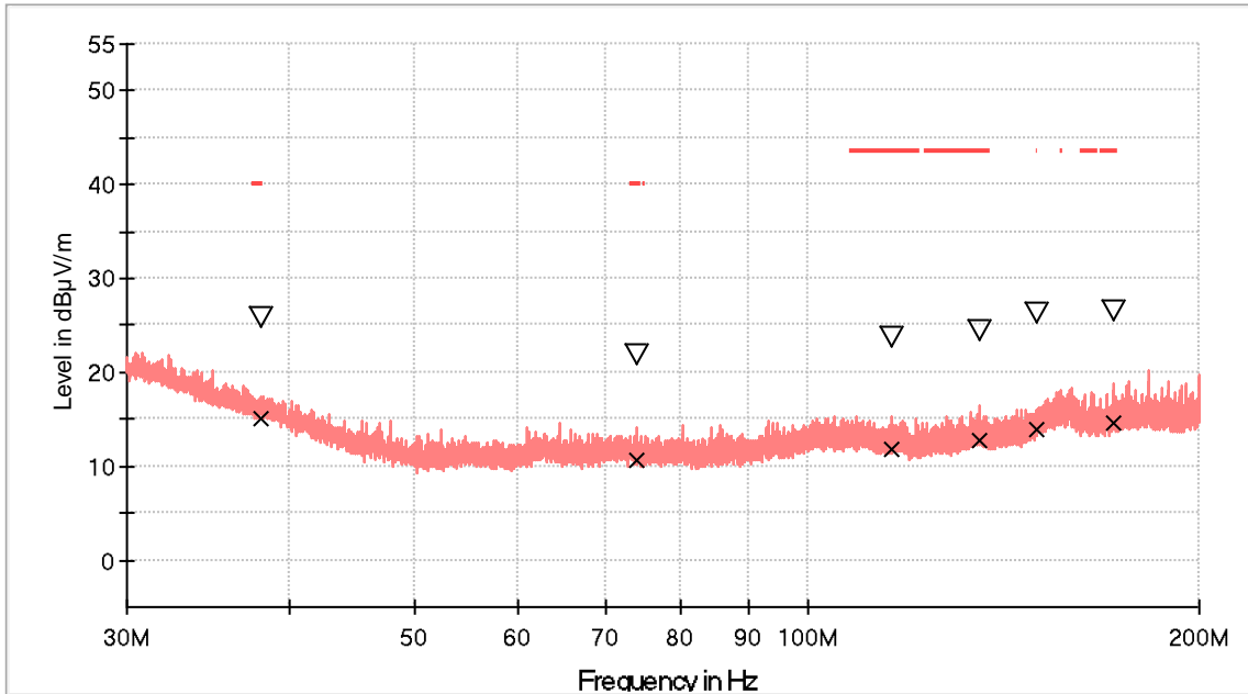
RF_FCC_15.225_E Field_30MHz_200MHz(SAC2)
