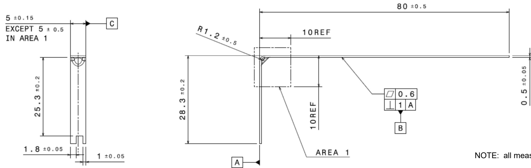
ANT1 && ANT2 && ANT3 (FO3-TR903BDA) Overview: [Dimensions in mm]
