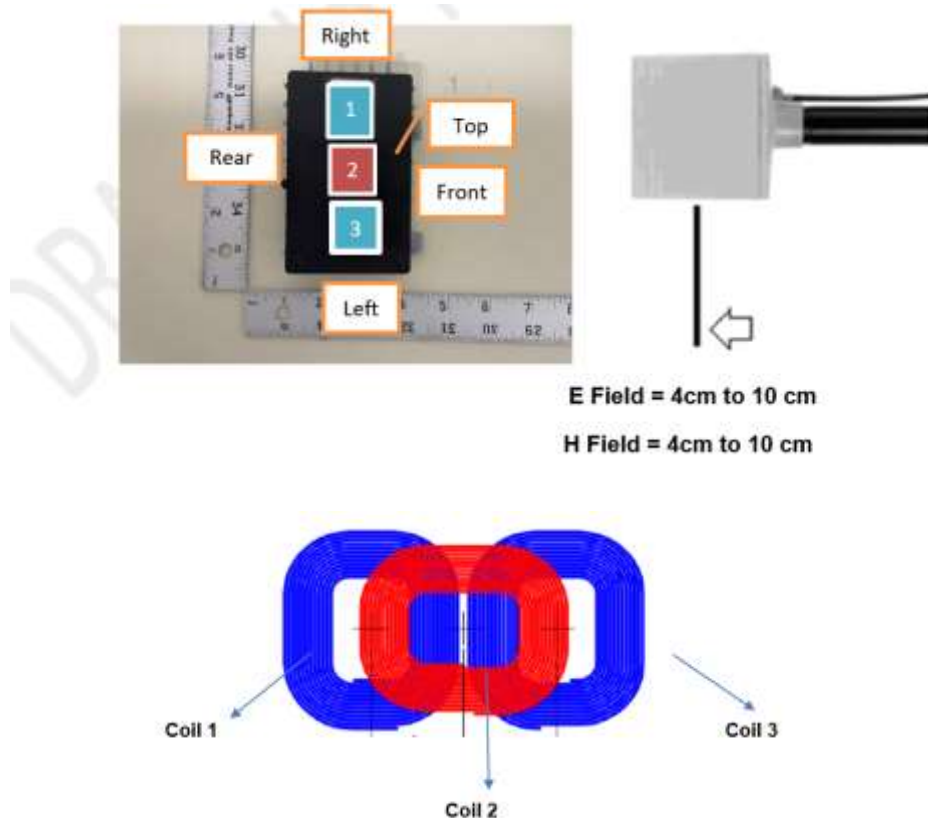
Figure 1: WPT measurement setup
