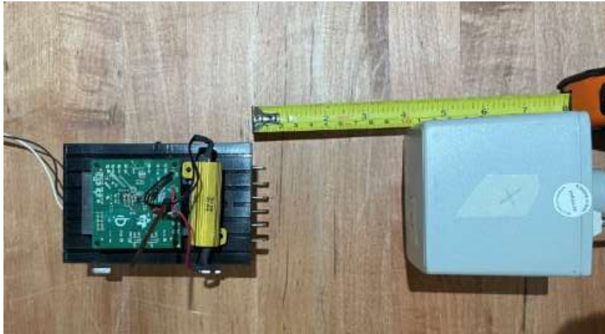
Figure E4. DUT Test setup 2
