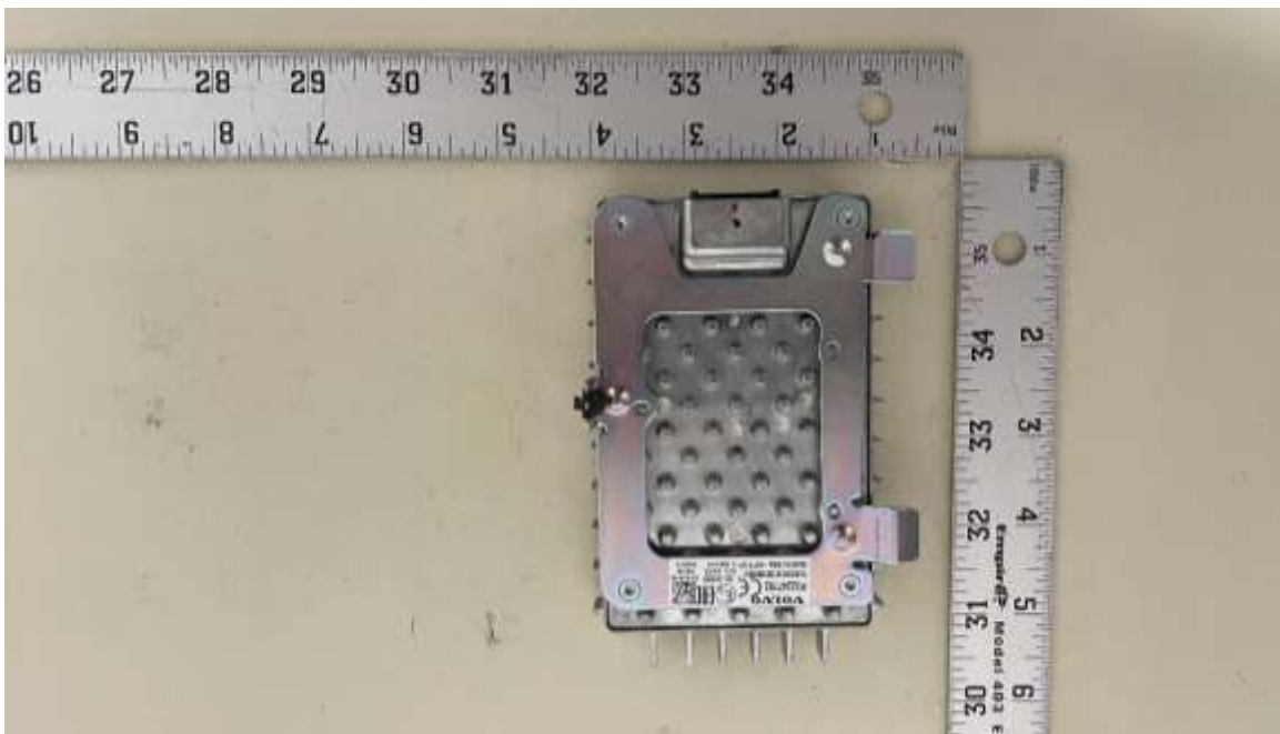
Figure B2. Bottom View of DUT
