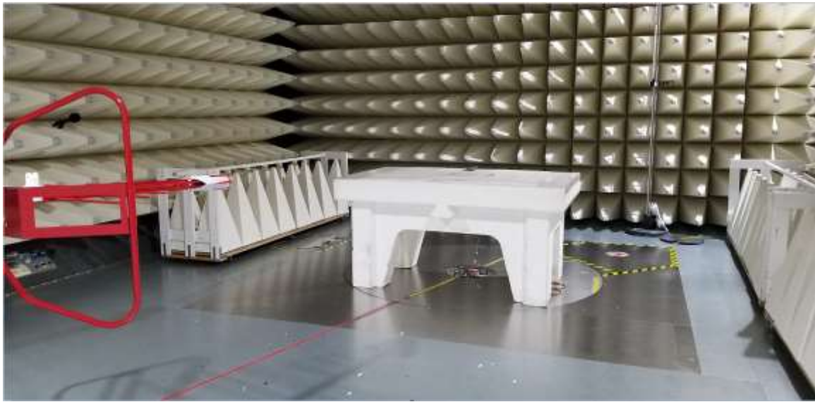
Figure B5. Low Range Radiated Emission test setup (30 MHz to 1 GHz)
