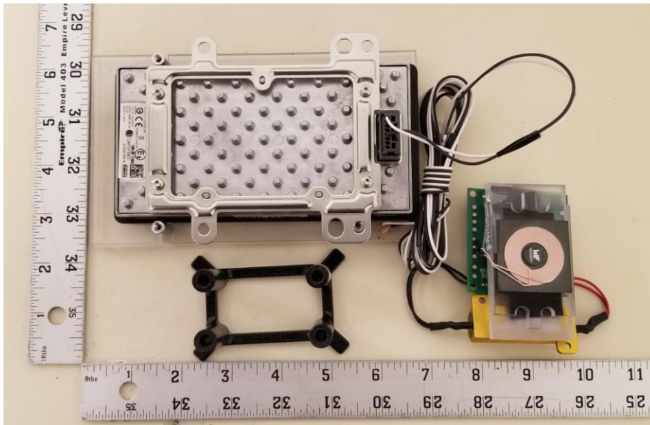
Figure B3. Rear View of DUT with load on the side
