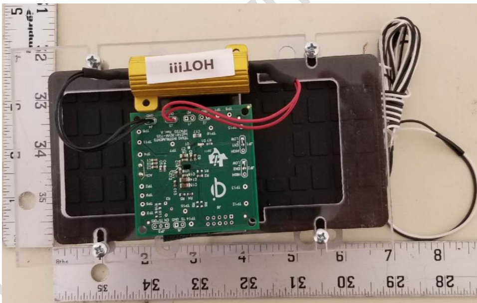
Figure B2. Front View of DUT with load
