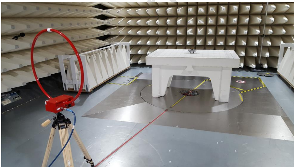
Figure B4. Low Range Radiated Emission test setup 9KHz to 30MHz
