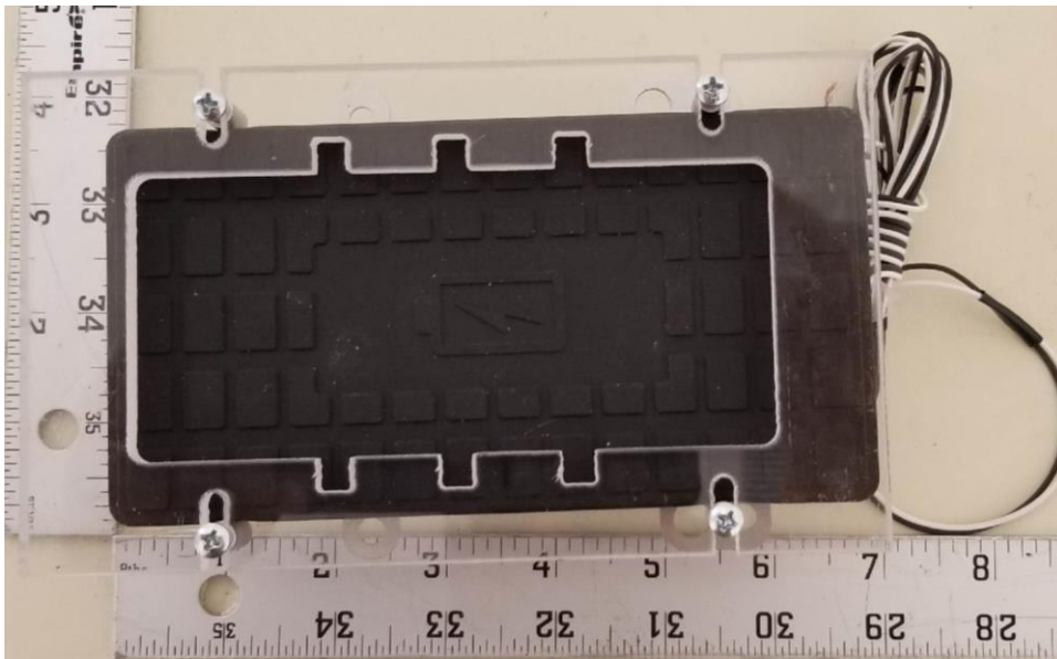
Figure B1. Front View of DUT with no load
