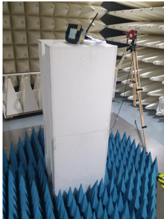
Figure B4. High Range Radiated Emission test setup using Horn antenna
