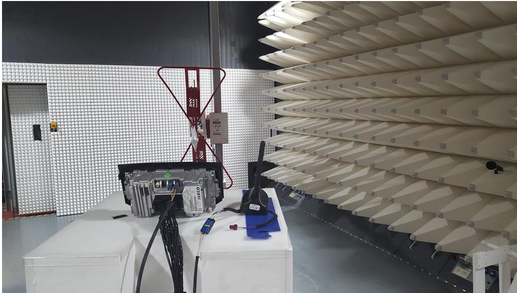
Figure B3: Low Range Radiated Emission test setup using Biconical antenna
