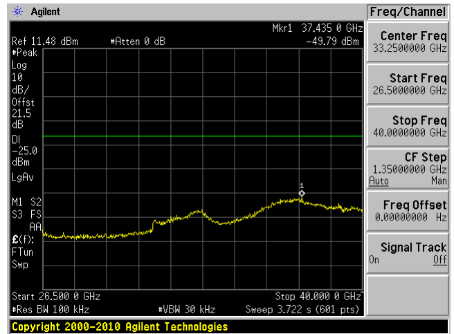
High Channel 5920 MHz Ant 2, 26.5GHz – 40GHz
