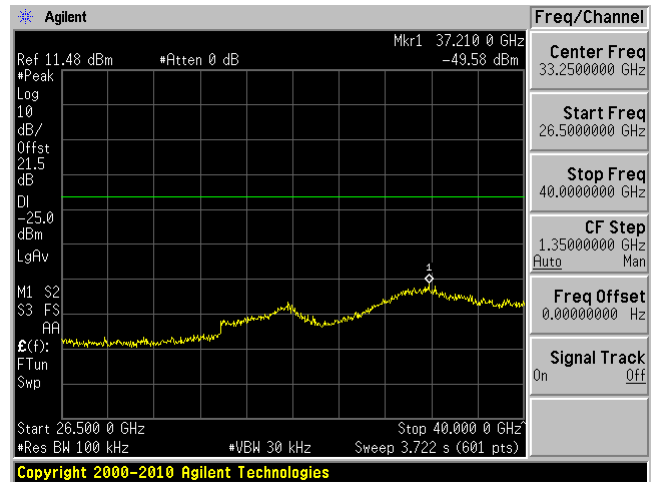
Low Channel 5860 MHz Ant 1, 26.5GHz – 40GHz
