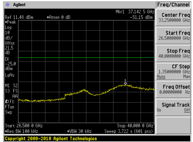
High Channel 5920 MHz Ant 1, 26.5GHz – 40GHz
