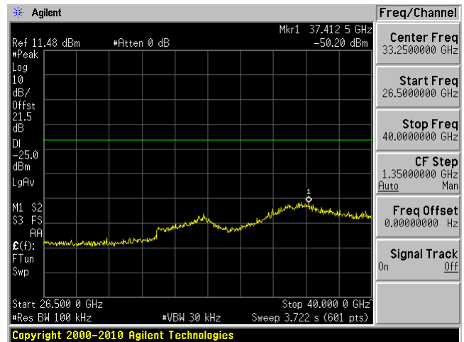
Low Channel 5860 MHz Ant 2, 26.5GHz – 40GHz
