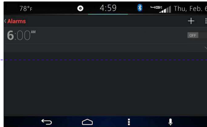
Figure 66 Alarm list
