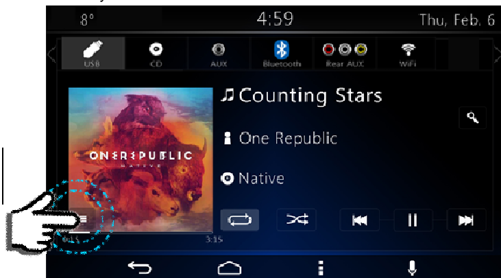
Figure 19: Views Softkey
