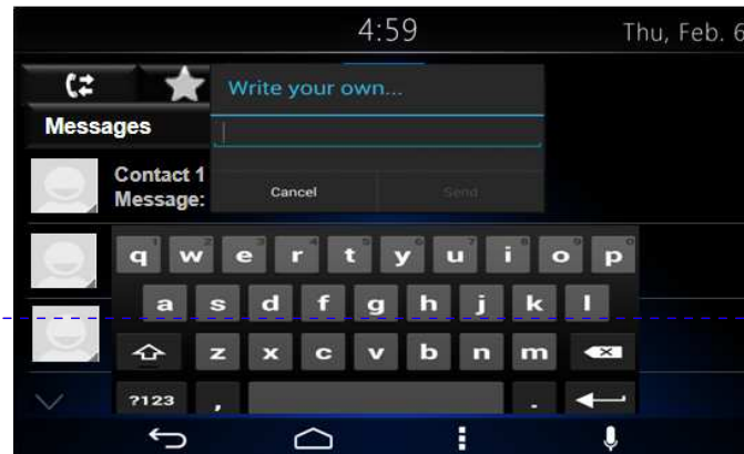
Figure 64 Message editor
