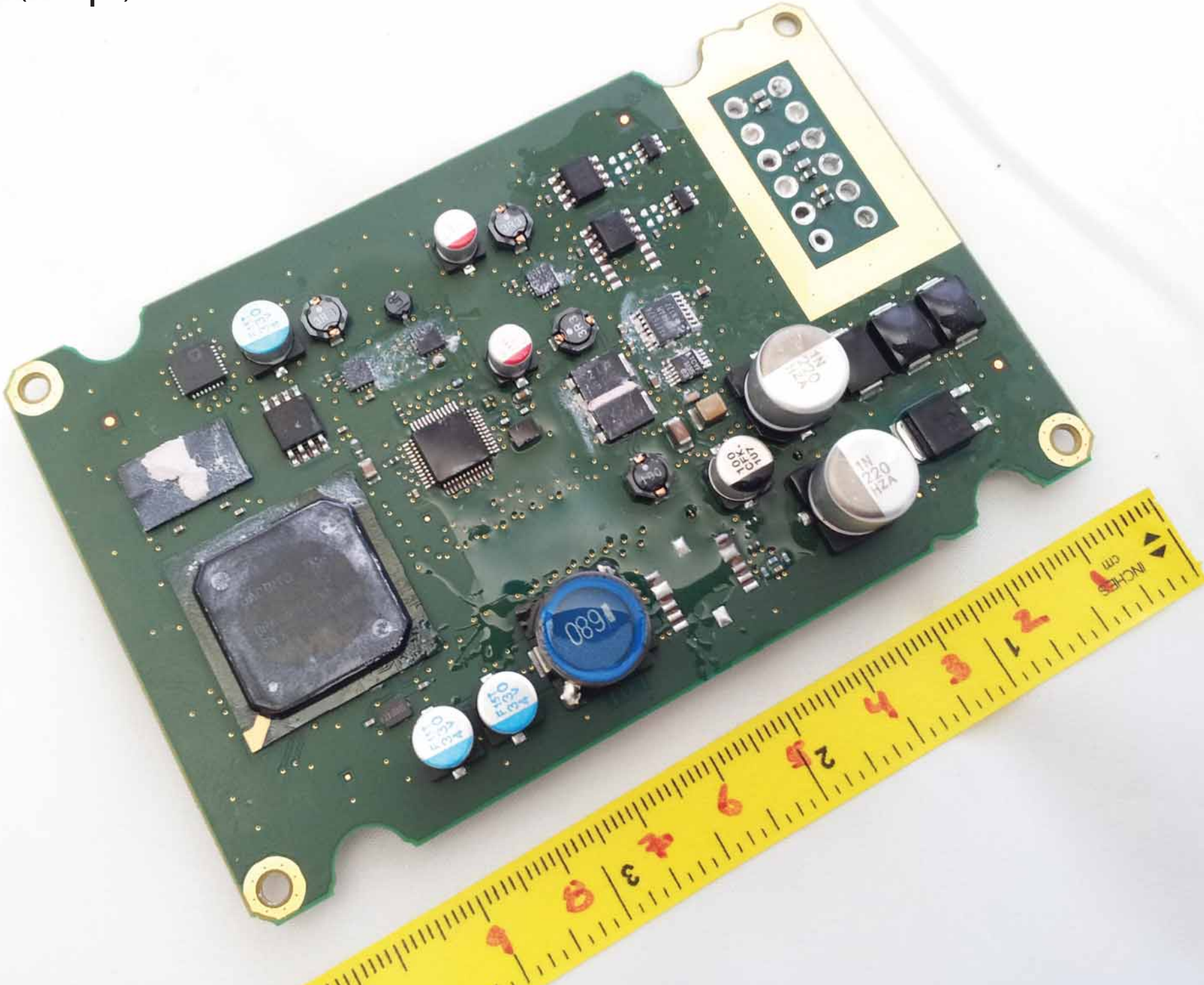
PCB (top)
