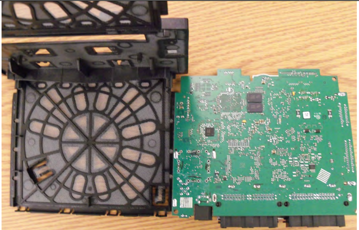
Bottom Components & Cover
