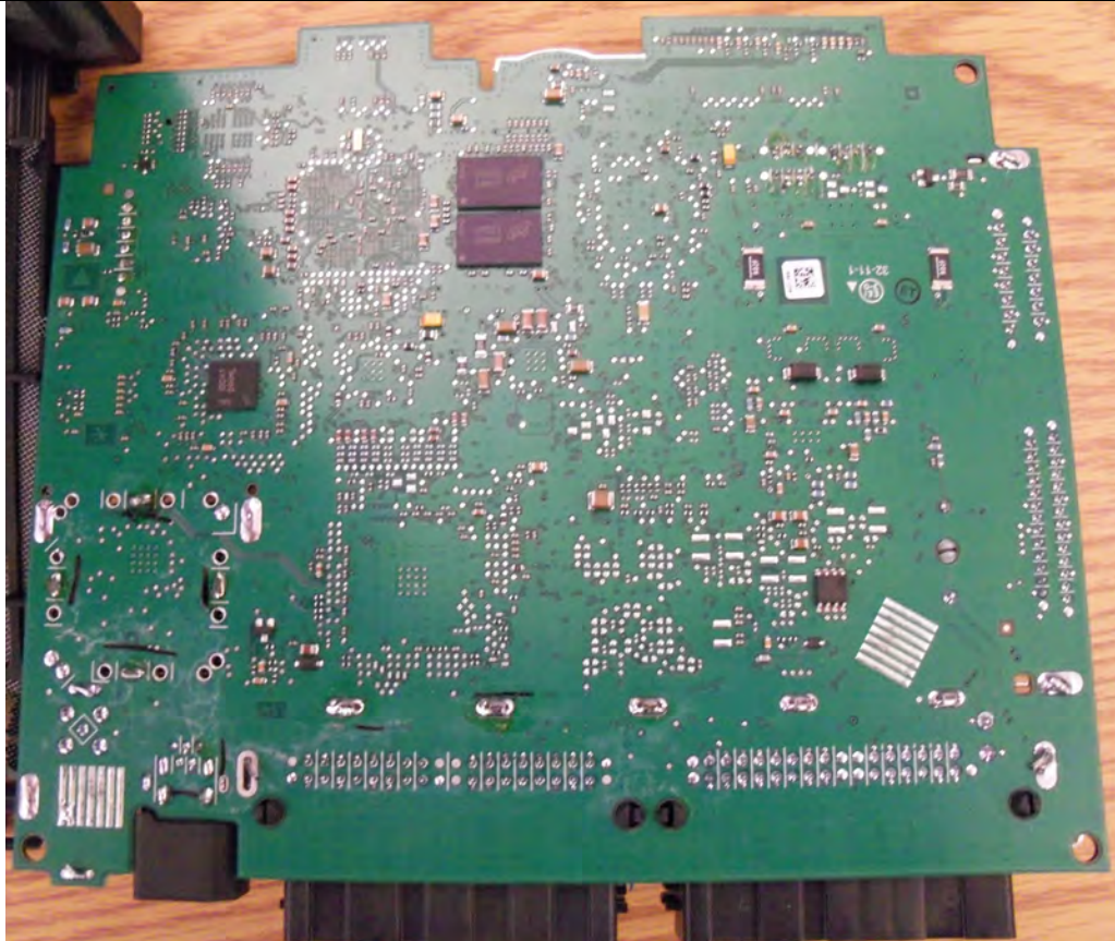
Bottom Components
