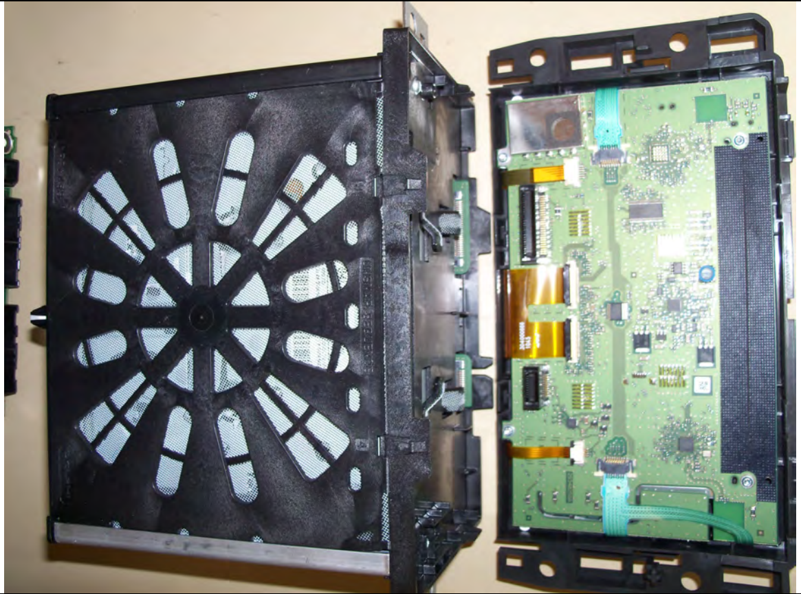
Faceplate & Keyboard
