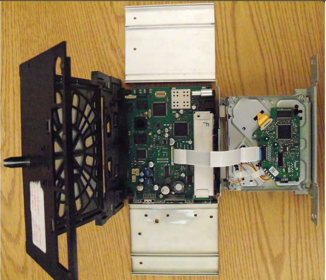
Mechanism & Top Components
