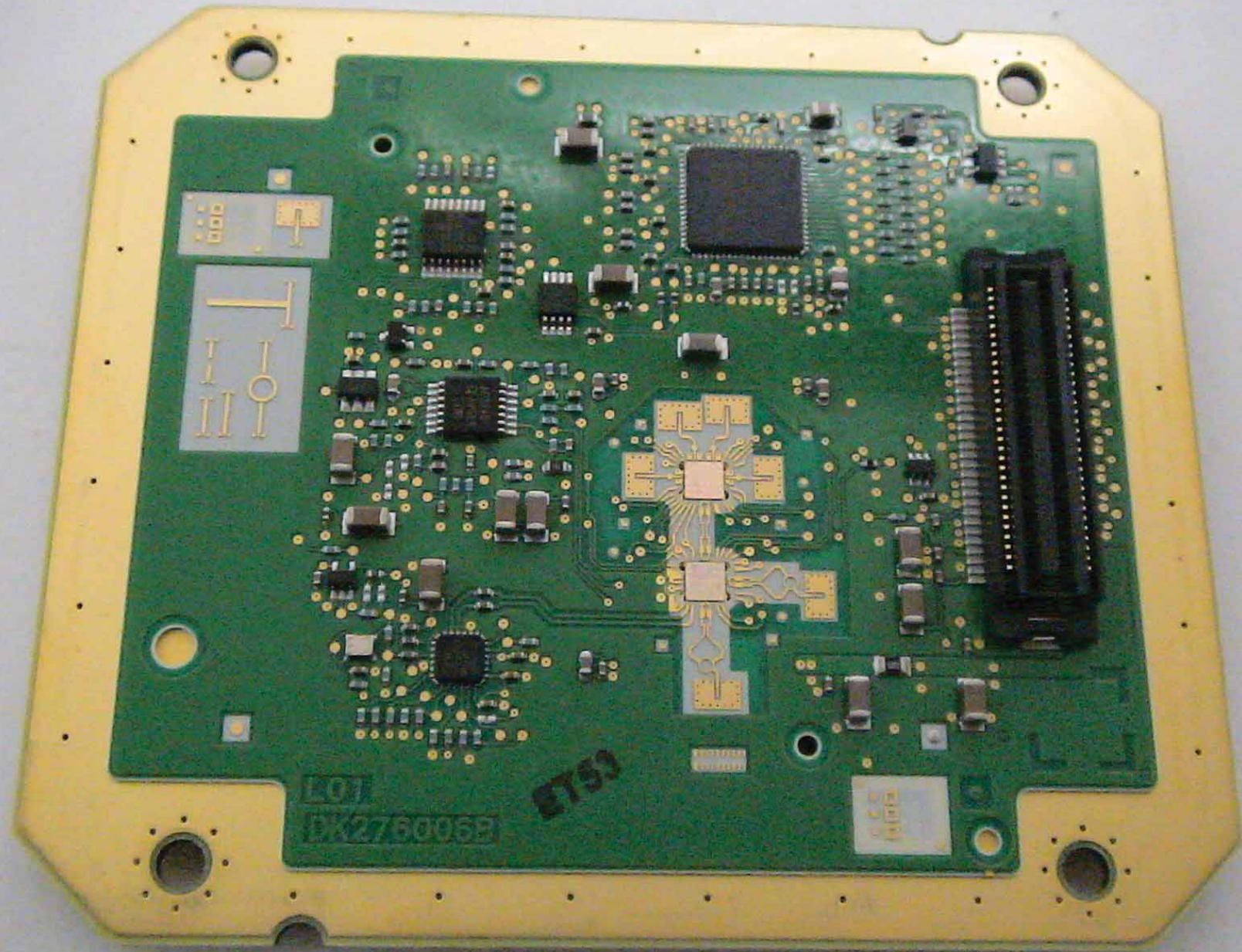
PCB (bottom)
