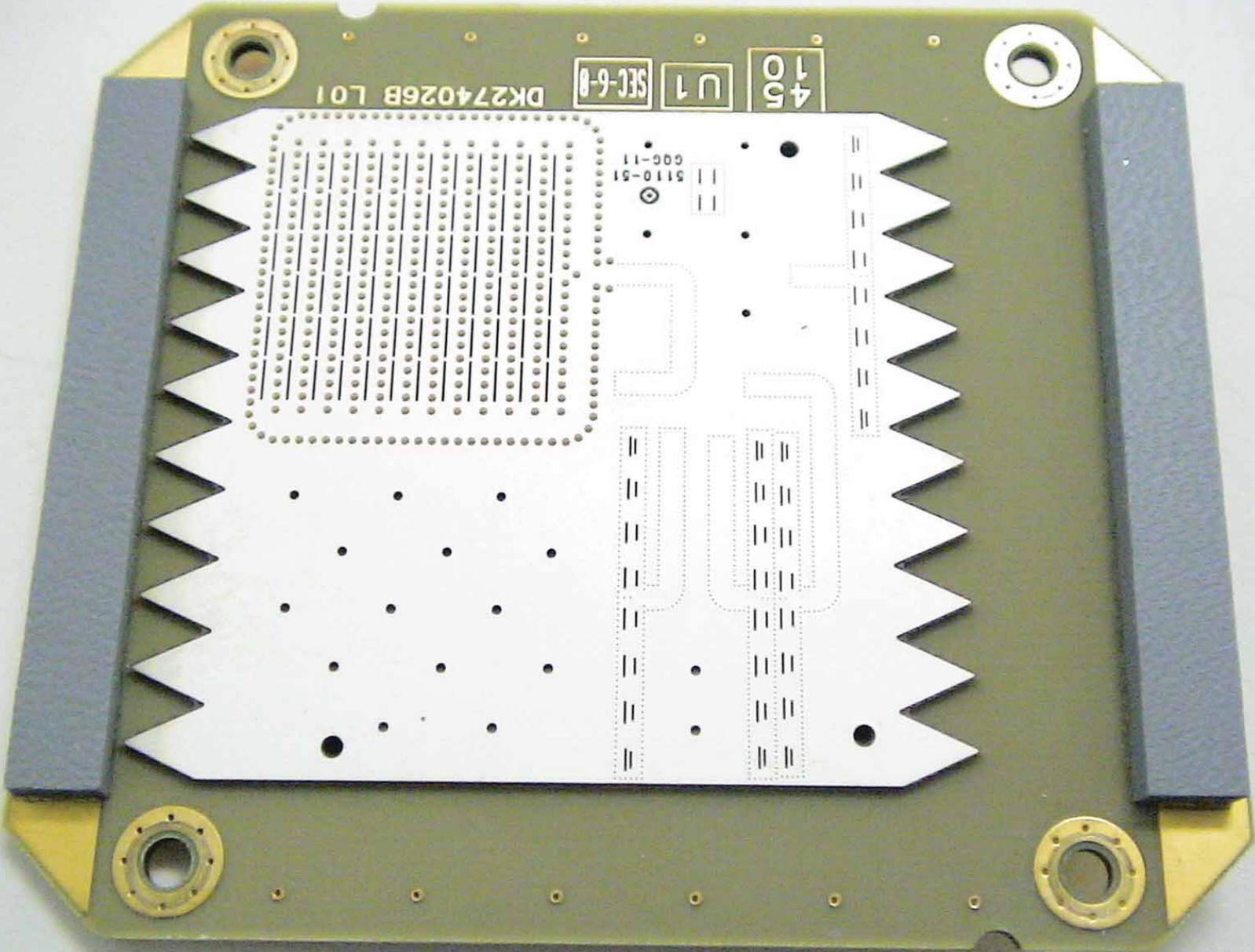
PCB (top)
