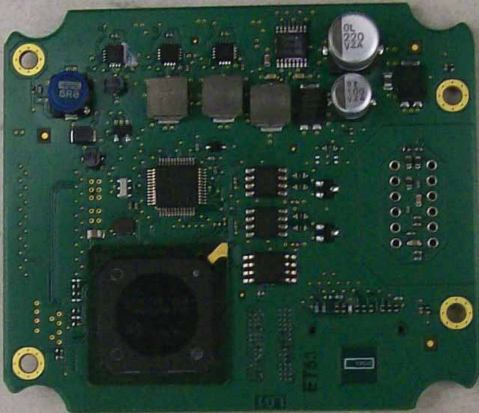
PCB (bottom)
