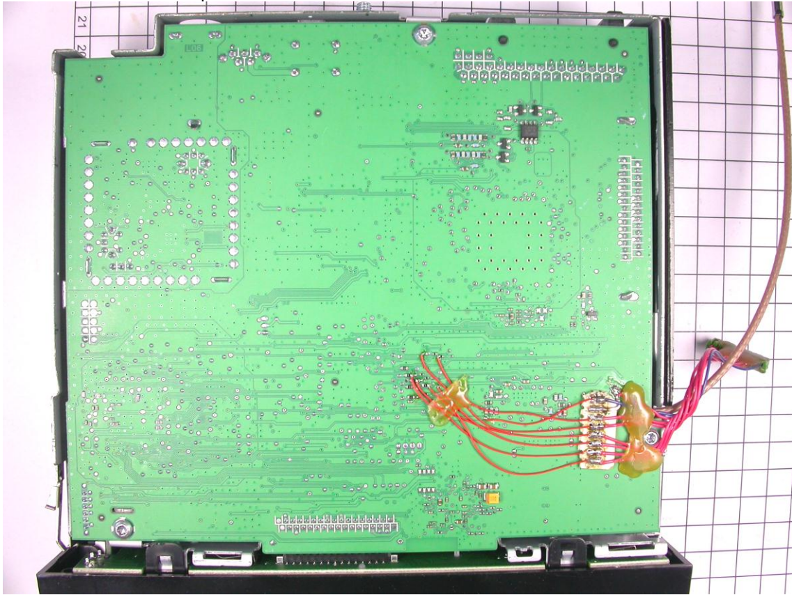
Motherboard with connection for special test mode control:
