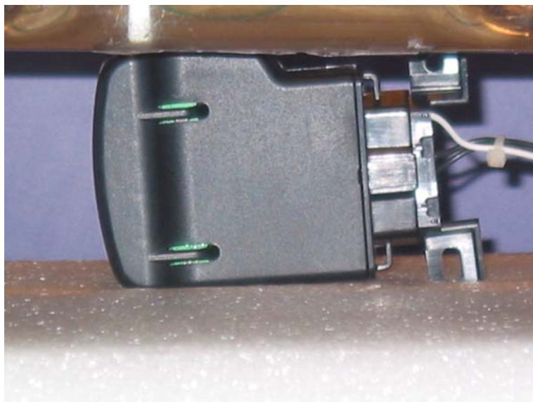
Side 'B' Test Position 0 mm Gap
