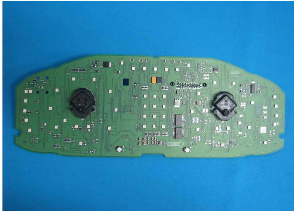
Cluster – Top View of PCB
