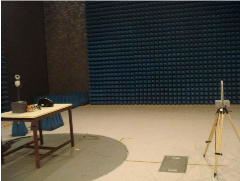
Test setup-Radiated Emissions Below 30 MHz
