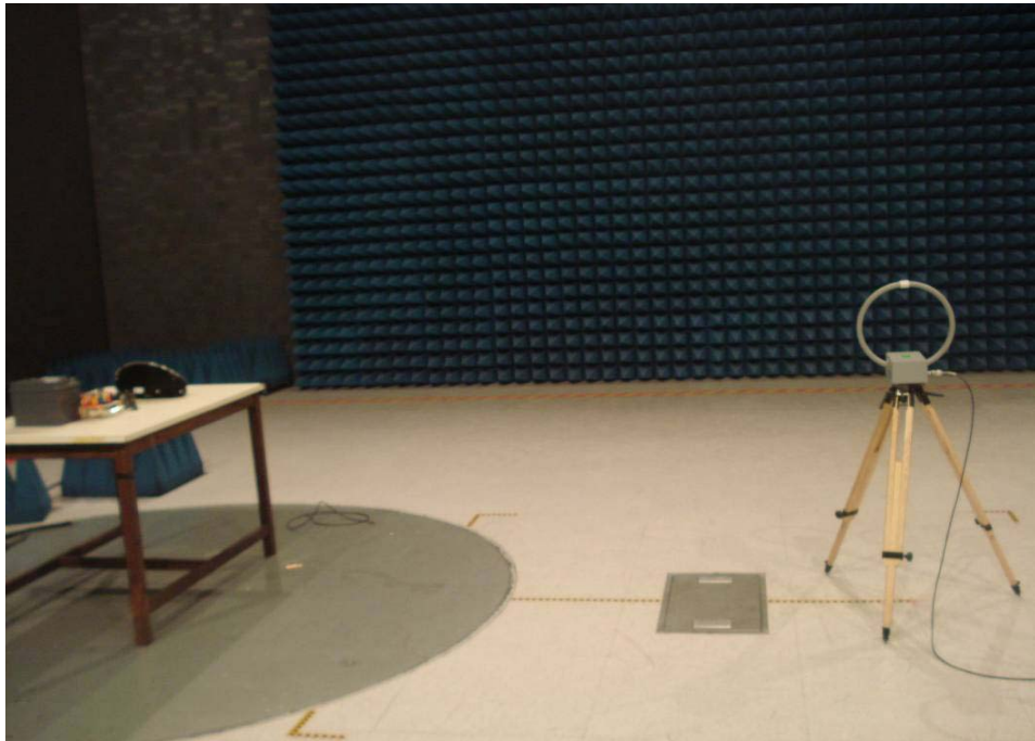
Test setup-Radiated Emissions Below 30 MHz
