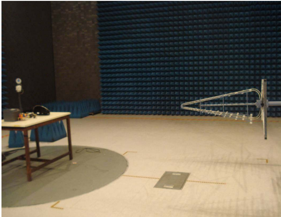
Test setup-Radiated Emissions Above 30 MHz
