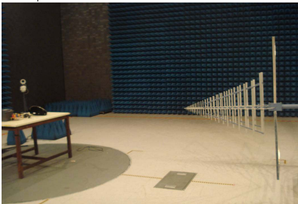
Test setup-Radiated Emissions Above 30 MHz
