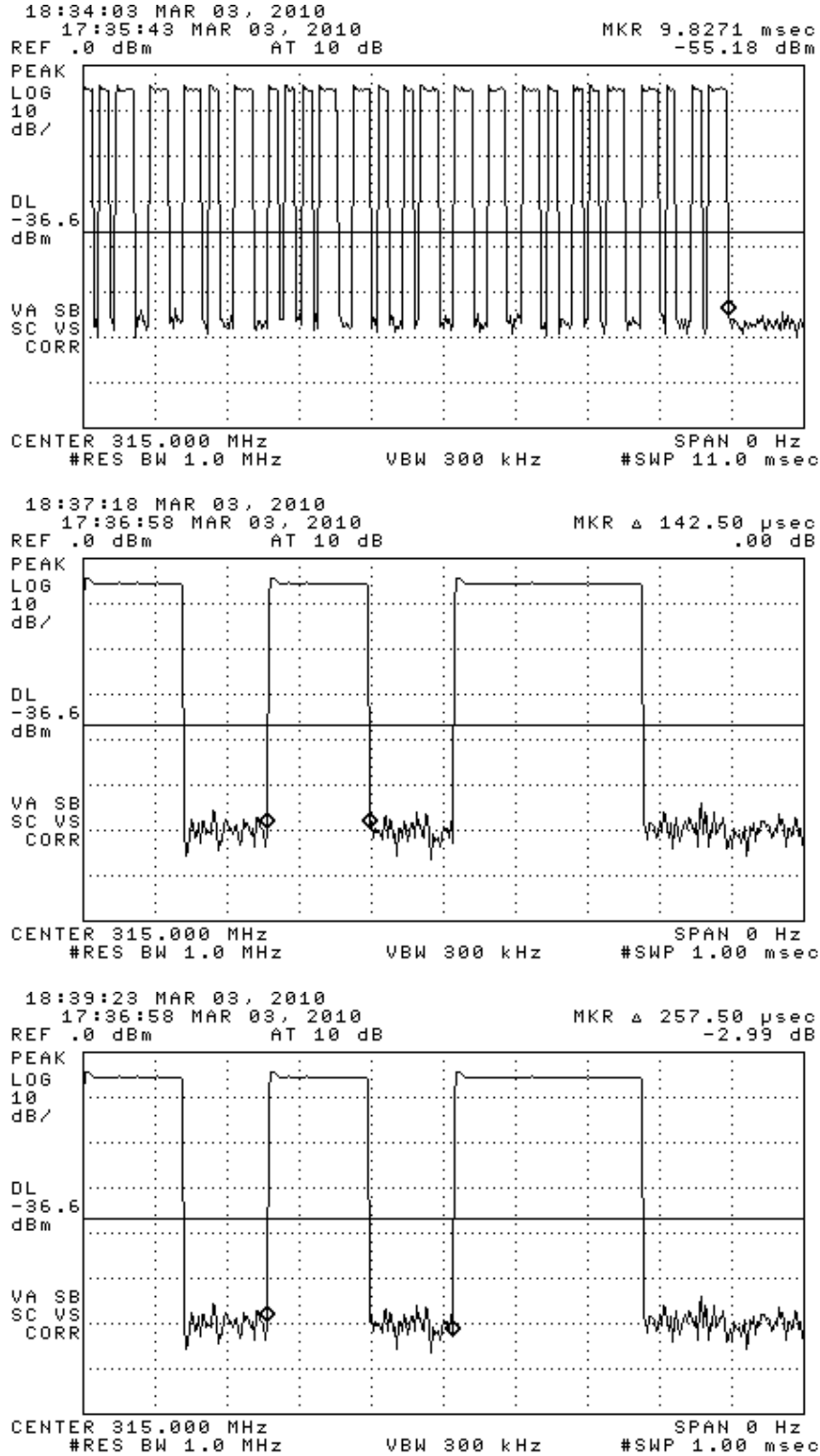
Figure 6.1(b). Transmission modulation characteristics. (top) expanded word showing Manchester encoding, (center) Manchester pulse width, (bottom) Manchester pulse period.
