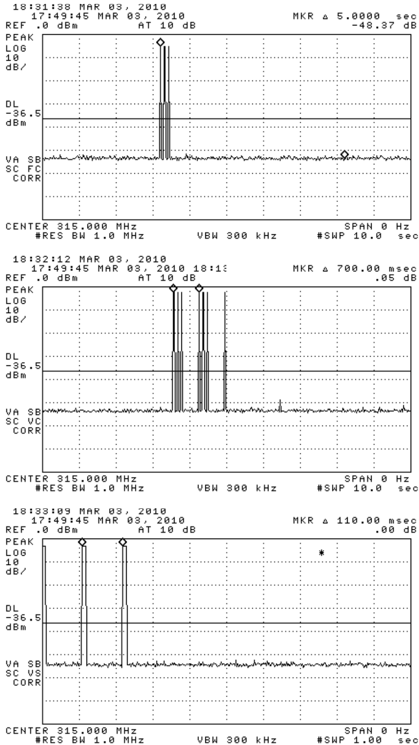
Figure 6.1. Transmission modulation characteristics. (top) transmission from single LF interrogation, (center) expanded transmission, (bottom) further expanded transmission.
