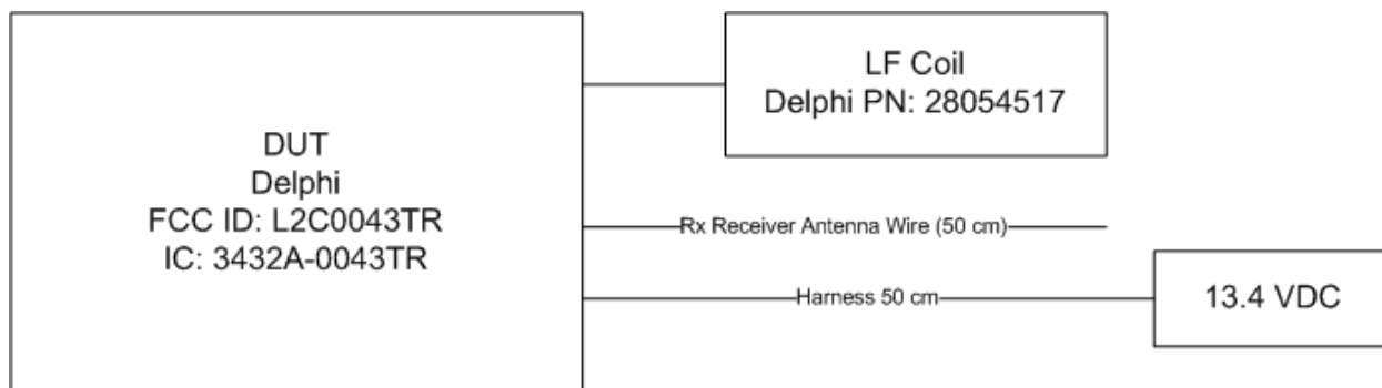
Figure 3.1 Block Diagram
