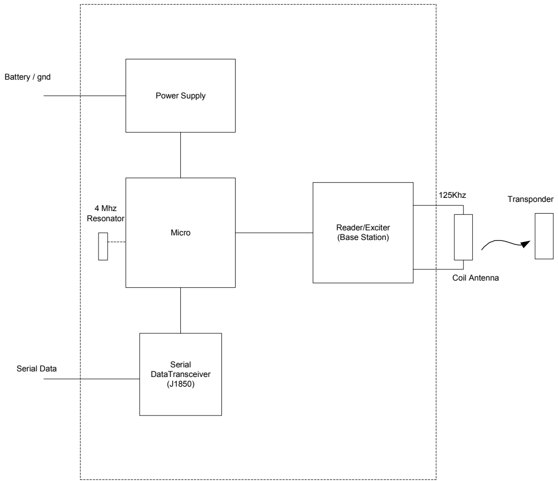
Block Diagram- Passey 3+
