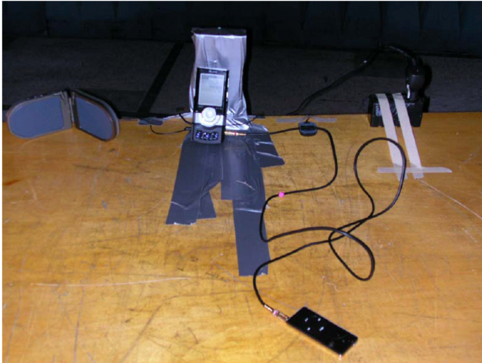
Photograph 4: Car Cradle Radiated Emissions Setup
