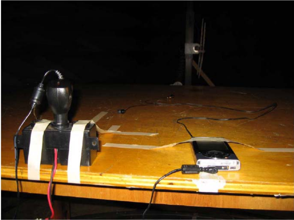
Photograph 6: Semi-Portable Radiated Emissions Setup
