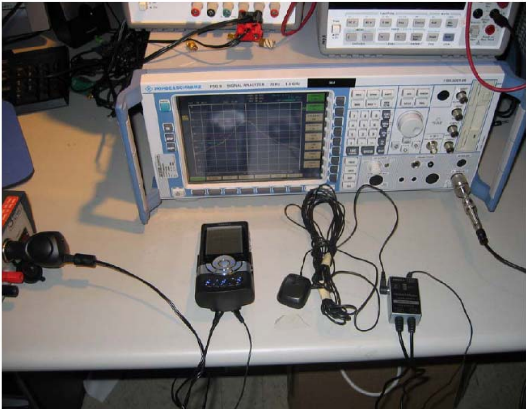
Photograph 11 : Occupied Bandwidth Setup
