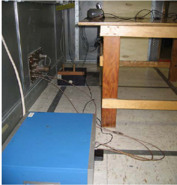
Photograph 1: Test Setup for Conducted Emissions
