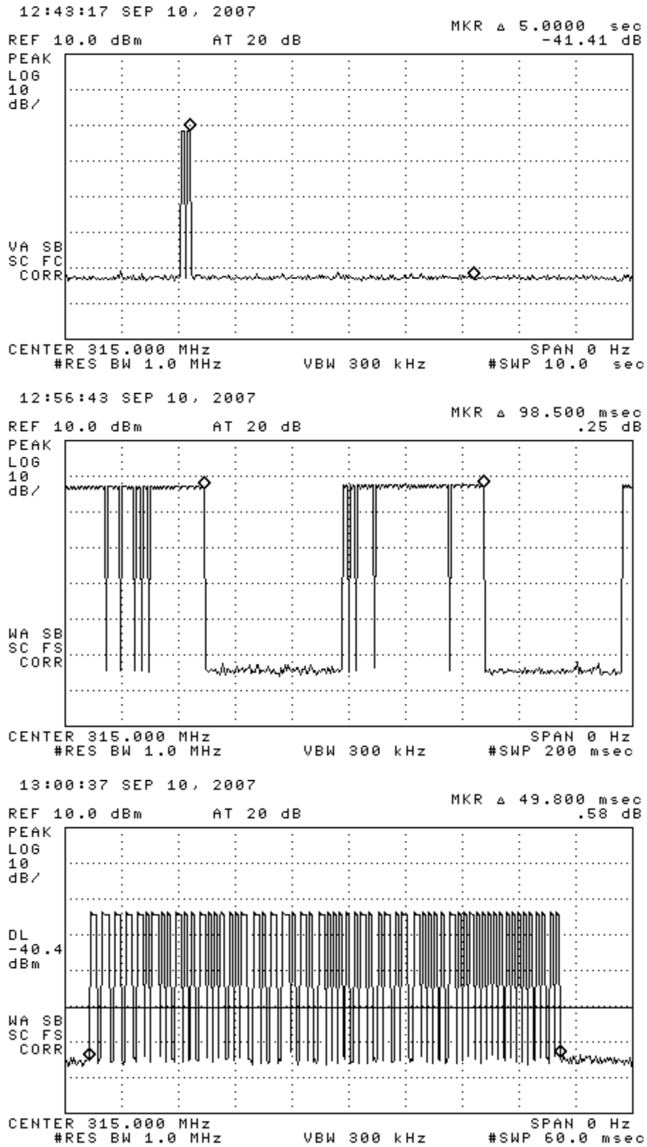
Figure 6.1(a). Transmissions modulation characteristics: (top) single button press, (center) repeated transmission, (bottom) expanded dataset.
