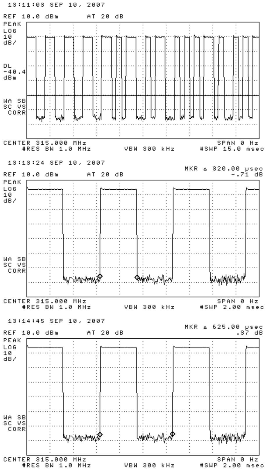
Figure 6.1(b). Transmissions modulation characteristics: (top) Manchester encoding, (center) pulse width, (bottom) pulse period.
