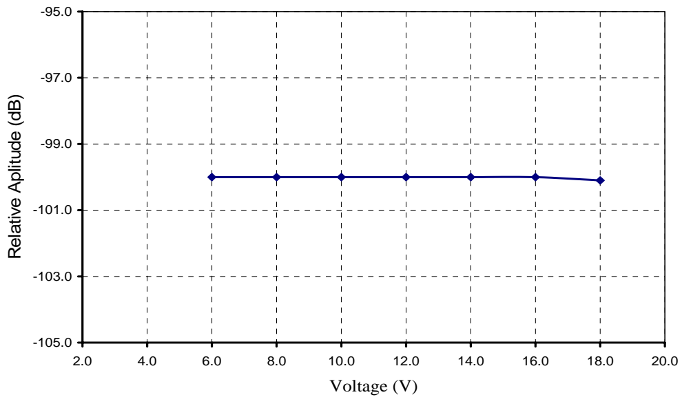
Figure 6.2. Relative emission at vs. supply voltage.
