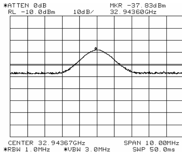
Figures 6.8-6.10. Receive Chain Emissions: RBW=1 MHz, VBW>RBW; measurement distance varied as necessary to maintain receive signal to noise ratio, peak detection, peak hold. Results reported in Table 6.2.
