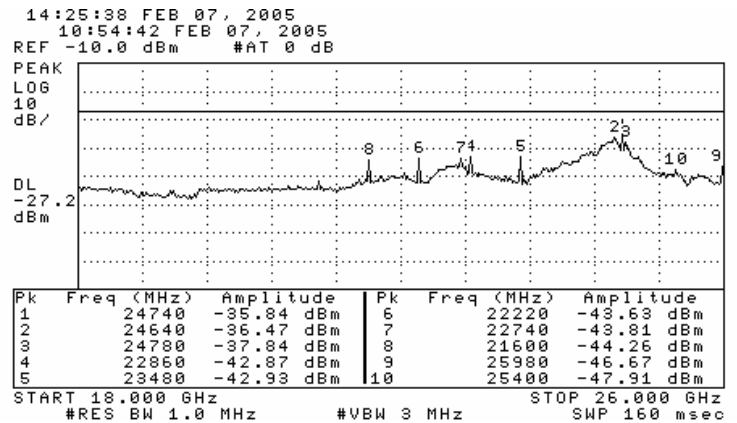
Figures 6.3-6.5. UWB Emissions: 9 kHz – 110 GHz (three example plots only). RBW=1 MHz, VBW>RBW; measurement distance varied as necessary to maintain receive signal to noise ratio, peak detect, peak hold. (Peak vs. RMS detection; see section 5.2 of this report.) All significant emissions reported in Table 6.1. Note 8.24 GHz emission is an emission from the receiver chain.
