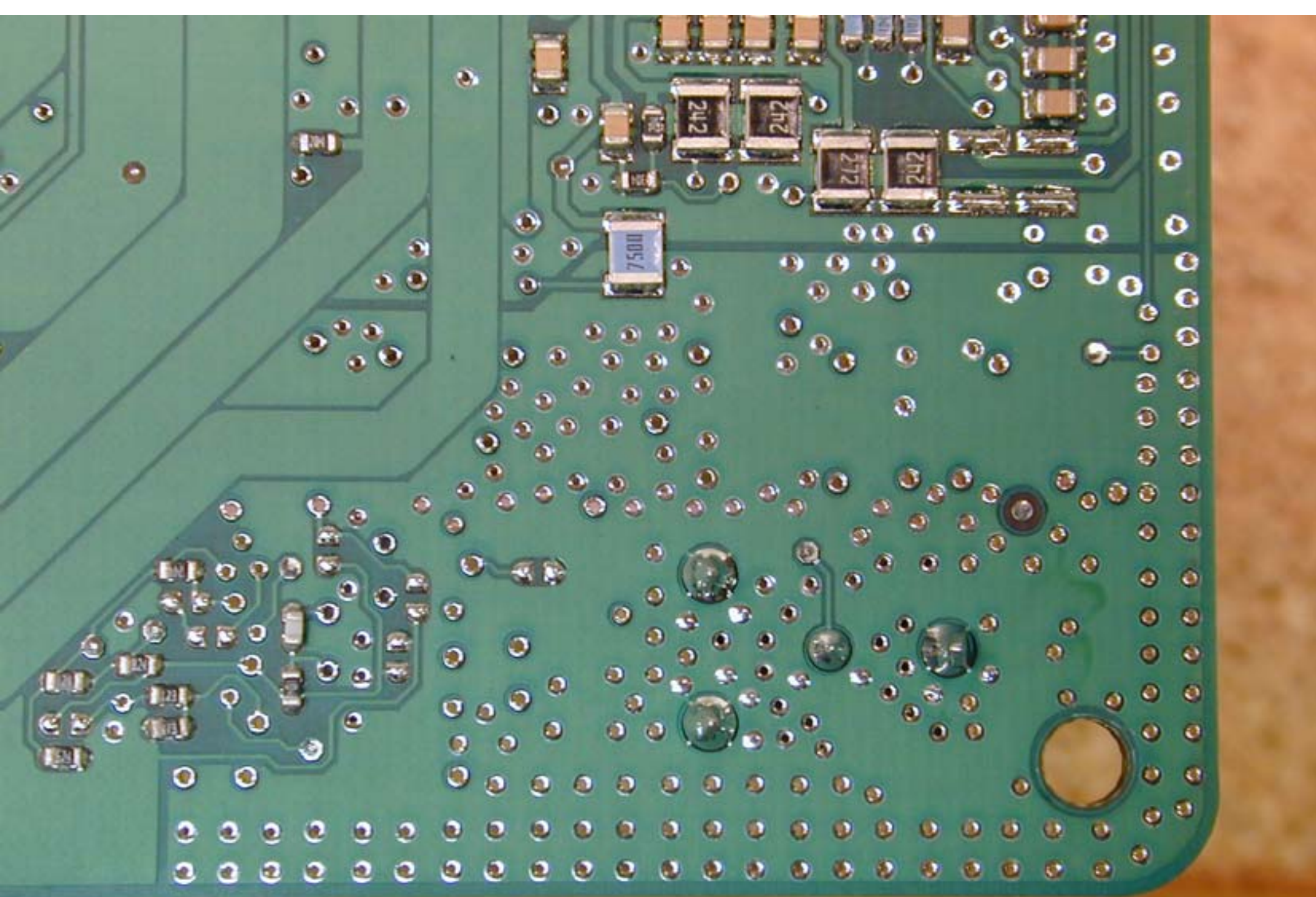
RF Section (bottom)
