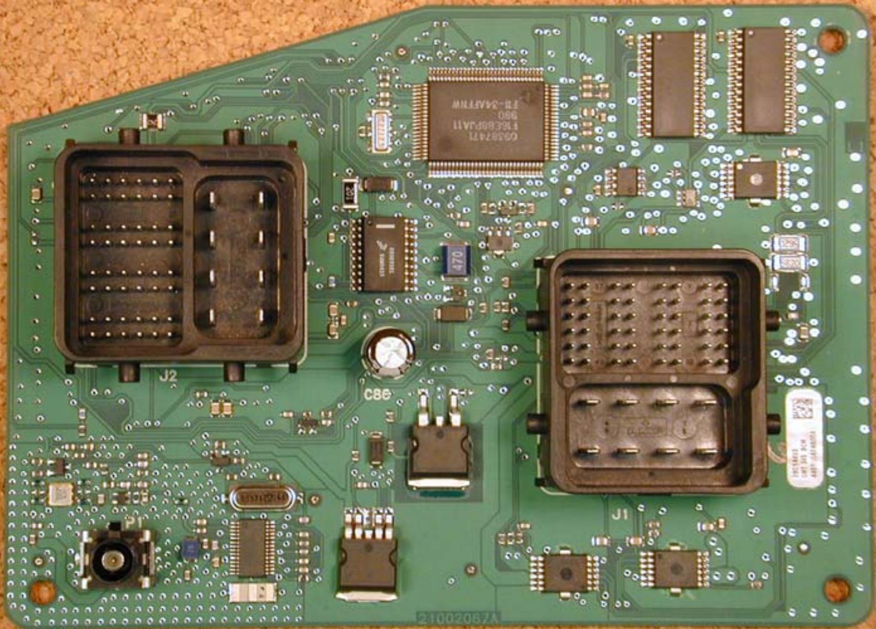
PCB (top)
