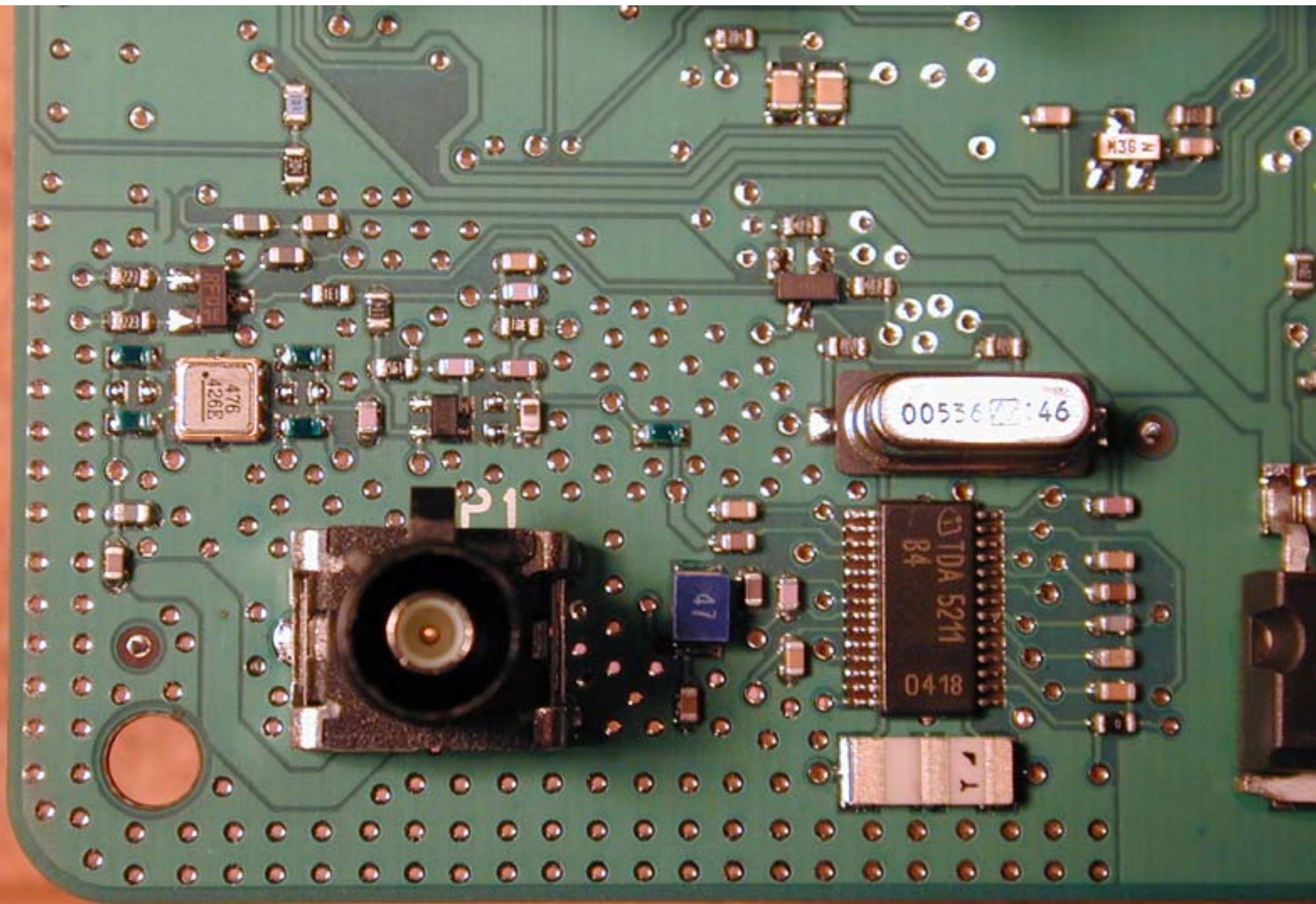
RF Section (top)
