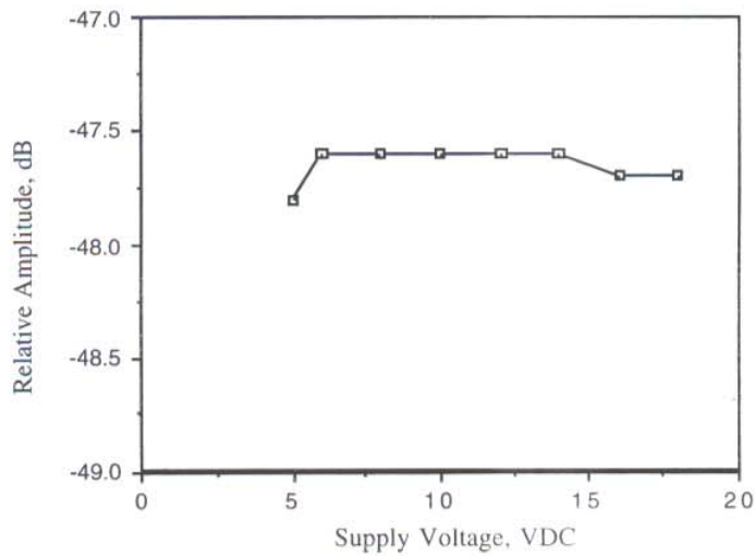
Figure 6.2. Relative emission at 651.4 MHz vs. supply voltage.
