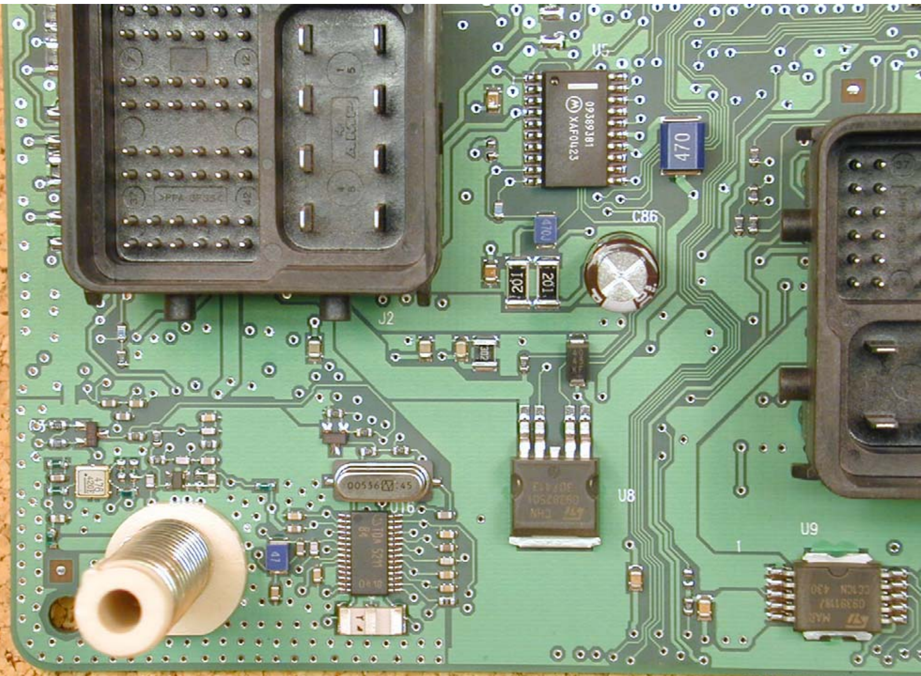
RF Section (top)
