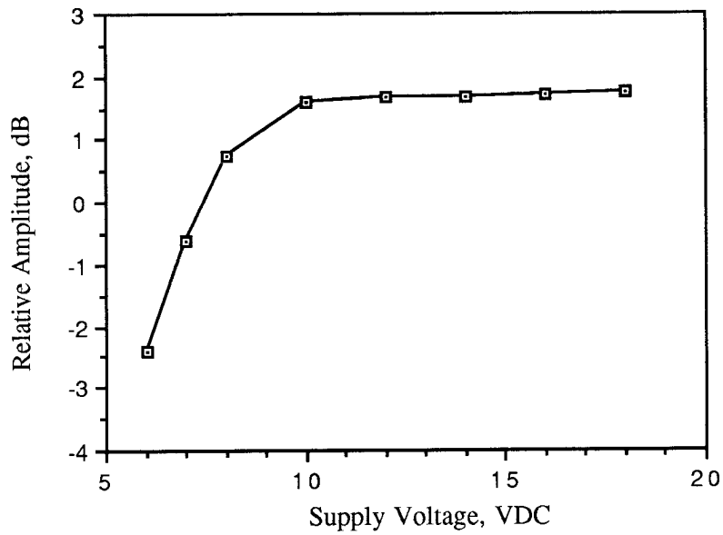
Figure 6.4. Relative emission at 132 kHz vs. supply voltage.
