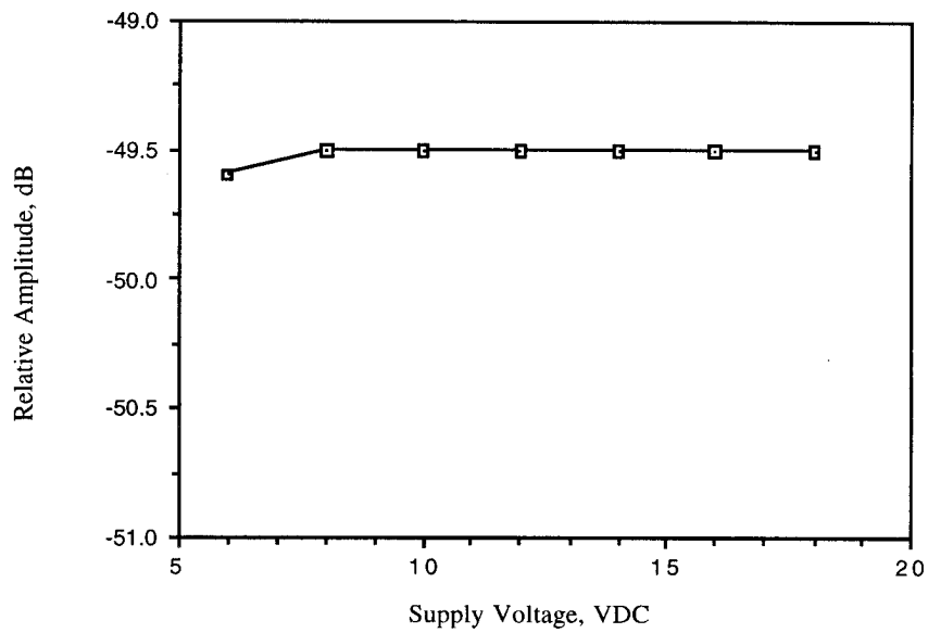
Figure 6.2. Relative emission at 651.4 MHz vs. supply voltage.
