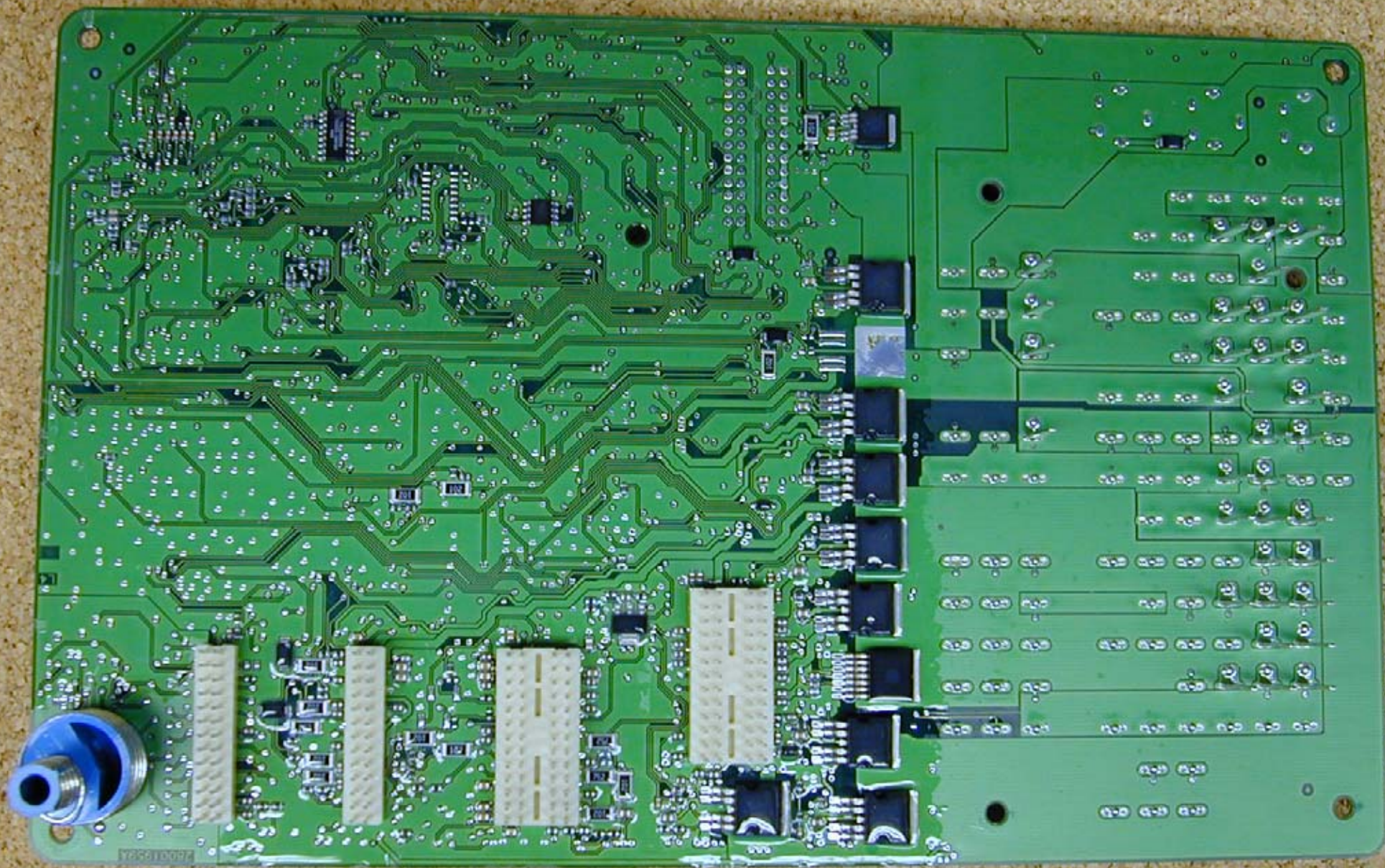
PCB (bottom)
