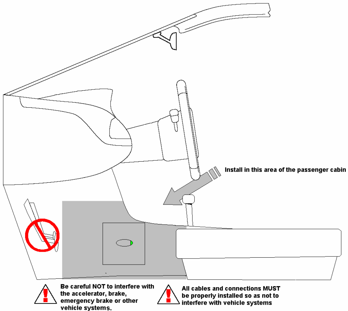
Figure 1 Vehicle with Center Console
