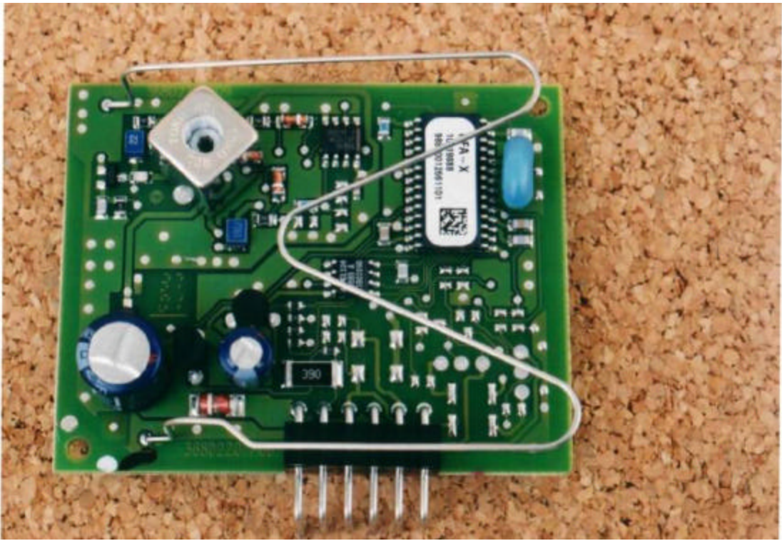
Receiver Board, top
