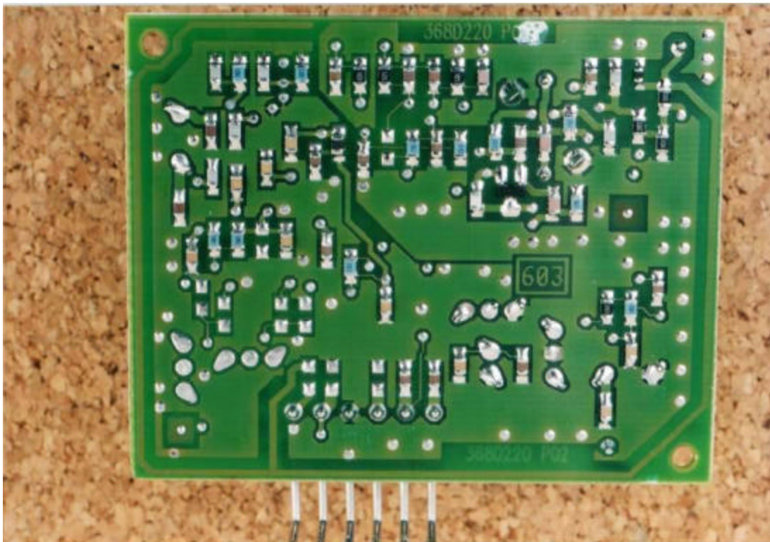
Receiver Board, bottom
