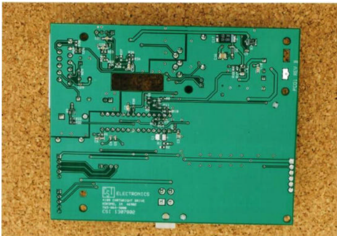
Mother Board, top
