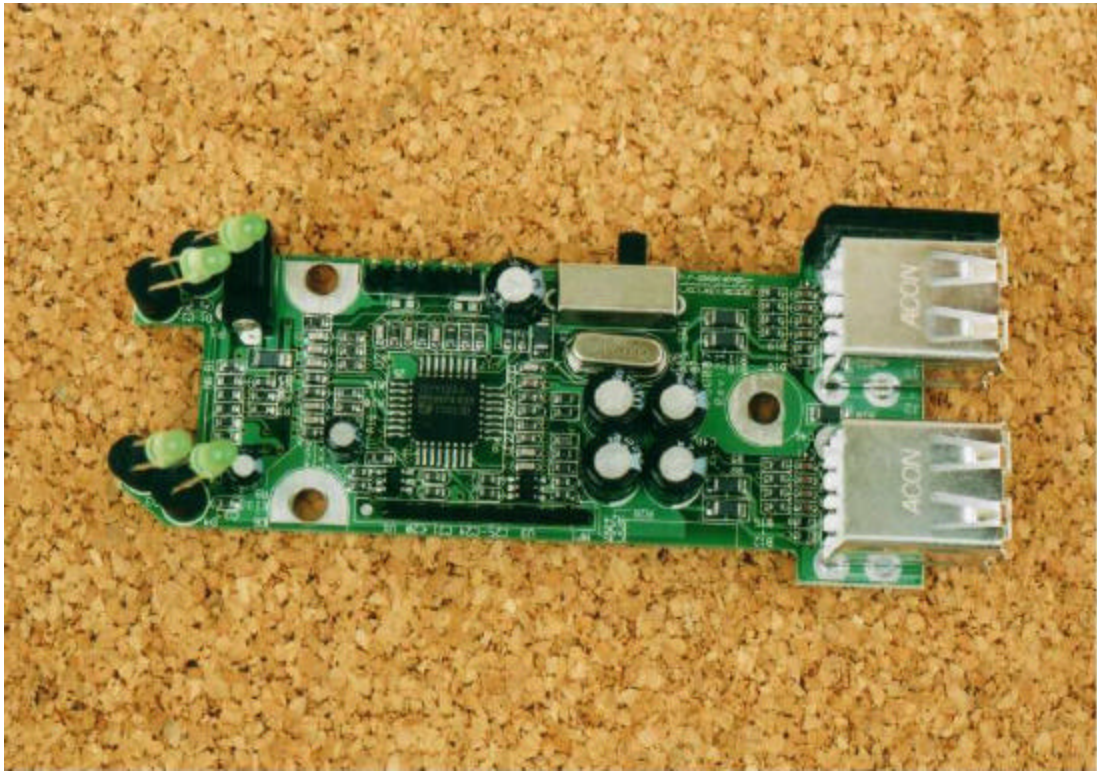
USB Board, top
