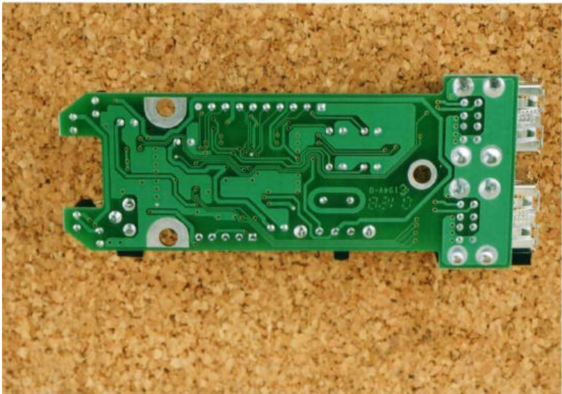
USB Board, bottom
