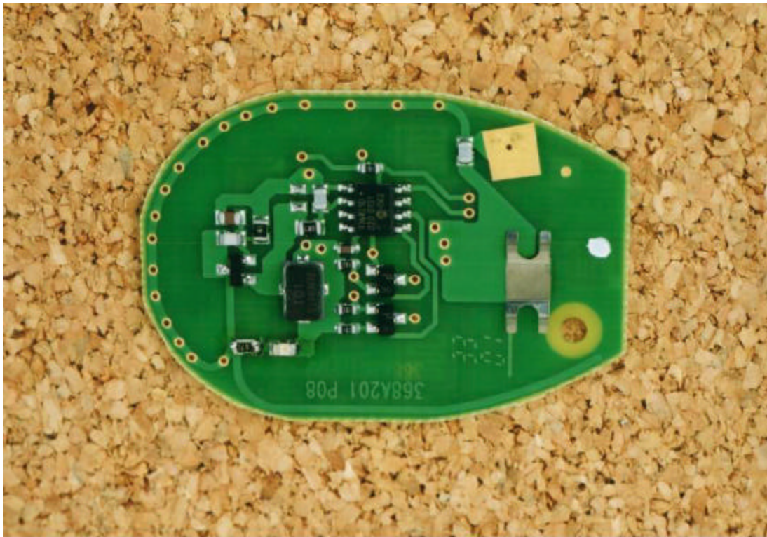
PCB, top
