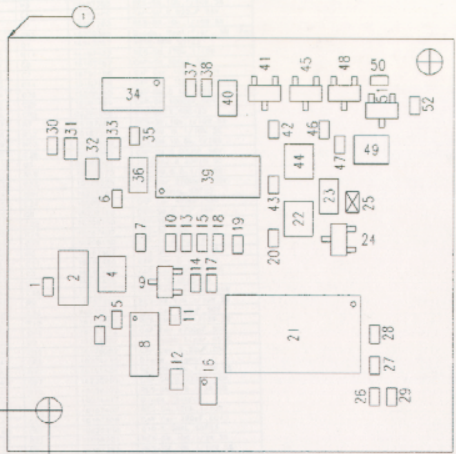
VIEWED FROM REFLOW SOLDER SIDE OF CIRCUIT BOARD
