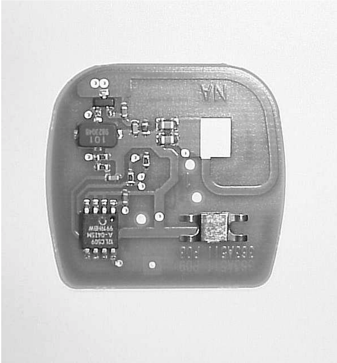
TSSM FOB Circuit Board Top View
