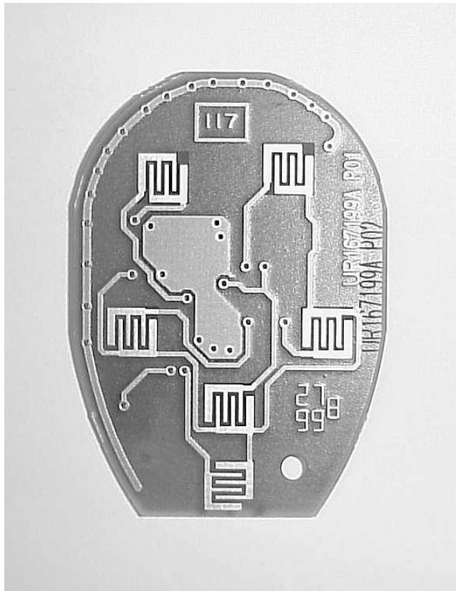
RFA-X FOB Circuit Board Bottom View
